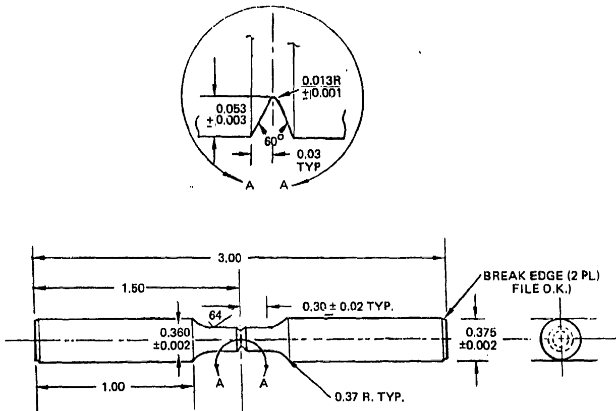
ROUND NOTCHED FATIGUE SPECIMEN ( K_t = 3 )
