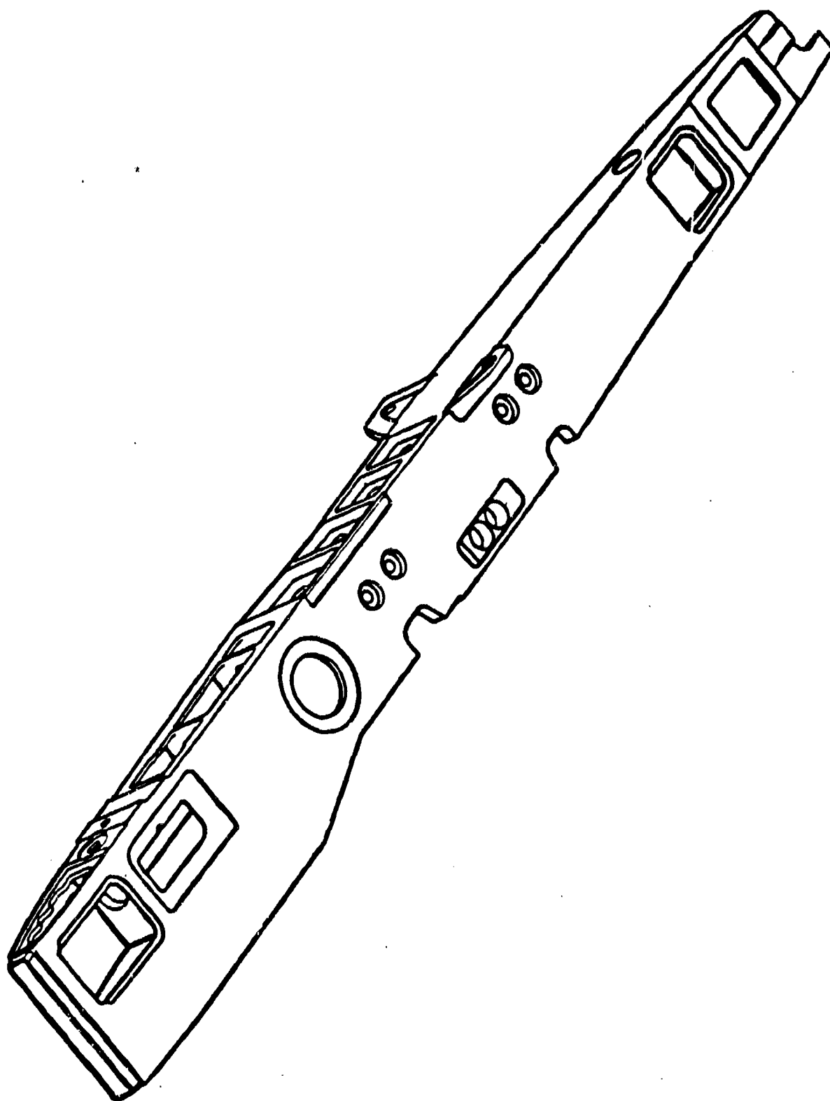
FIGURE 133. PYLON ASSEMBLY, MACHINE HOGOUT DESIGN, 7075 HAND FORGING
