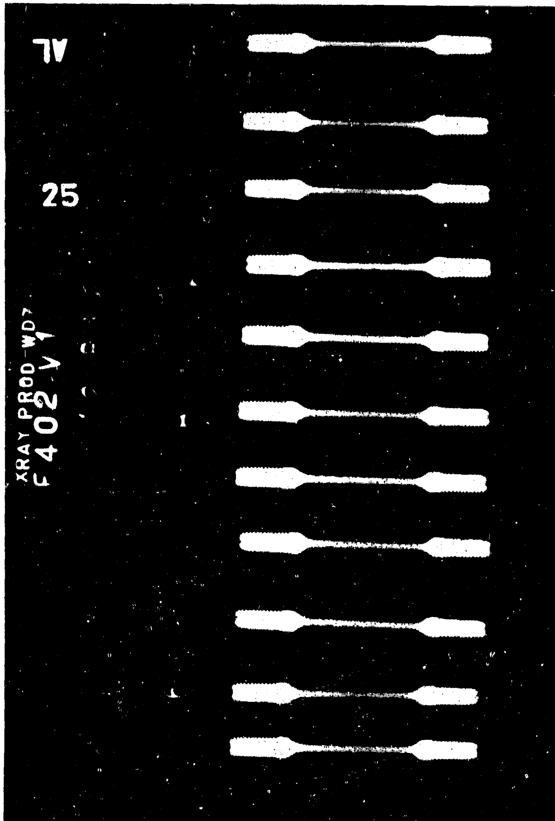
FIGURE 117. PHOTOGRAPHIC REPRODUCTION OF RADIOGRAPH SHOWING ROUND GAS POROSITY EVALUATED IN A201-T7 TENSILE SPECIMENS
