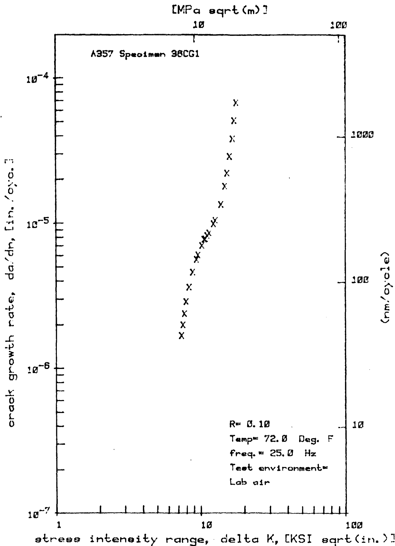
Figure 2. Fatigue crack growth plot of A357-T6 Specimen 36CG1.
