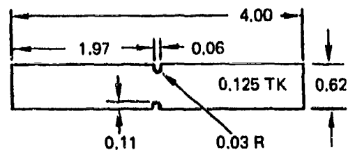
FLAT NOTCHED FATIGUE SPECIMEN ( K_t = 3 )
