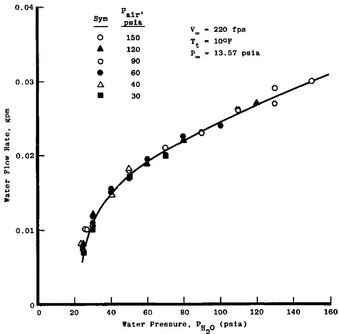
Figure 17. Water flow calibration, SS \frac{1}{4} J-1A Nozzle.
