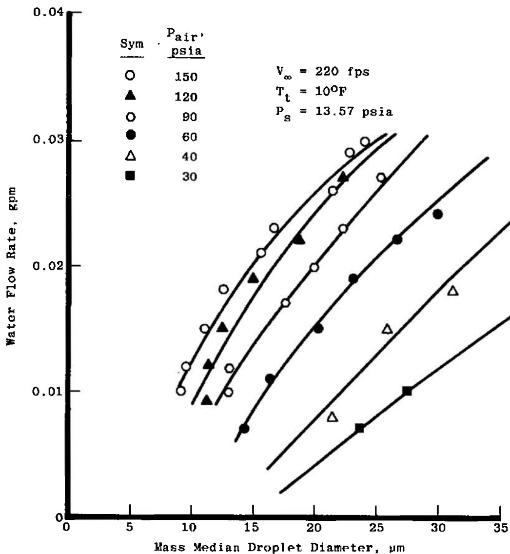
Figure 16. Droplet size calibration, SS \frac{1}{4} J-1A Nozzle.
