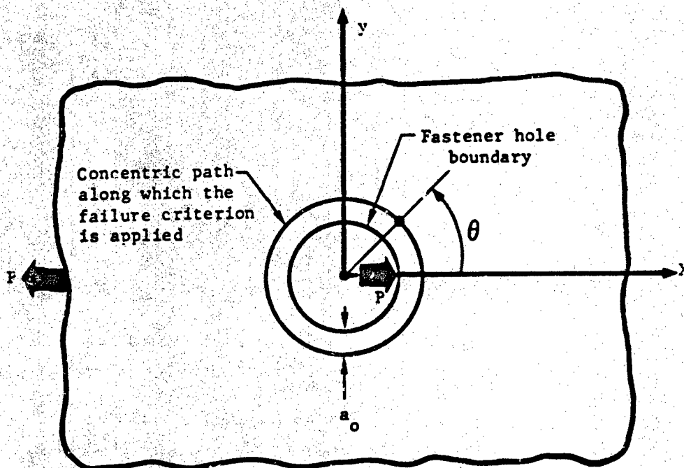
Figure 4-7. The Characteristic Distance ( a_0 ) Defining the Region Where the Maximum Strain, Hoffman or Hill Criterion is Applied.
