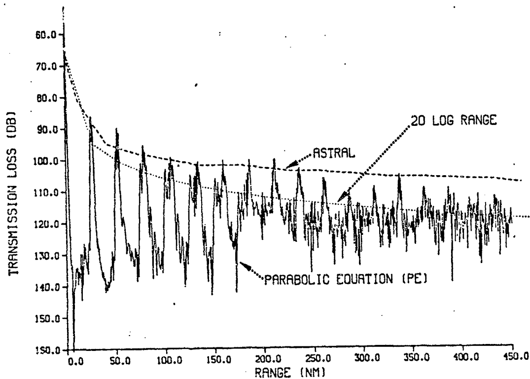
Figure 2.3 Comparison between ASTRAL and PE TL Models
