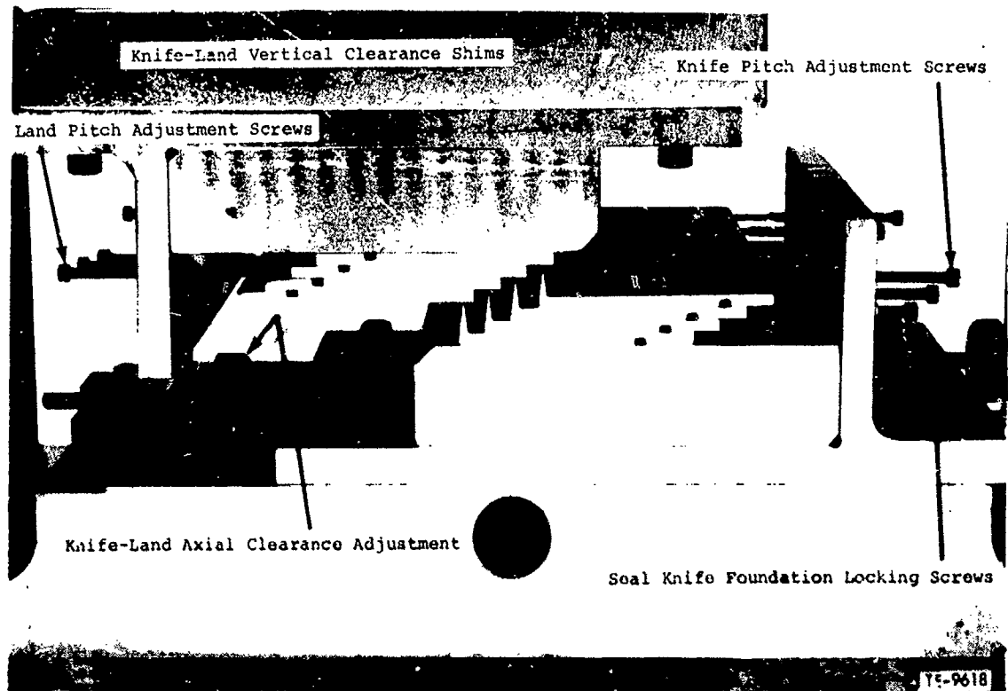
Figure 18. Two-dimensional (2-D) labyrinth seal rig with stepped seal installed.
