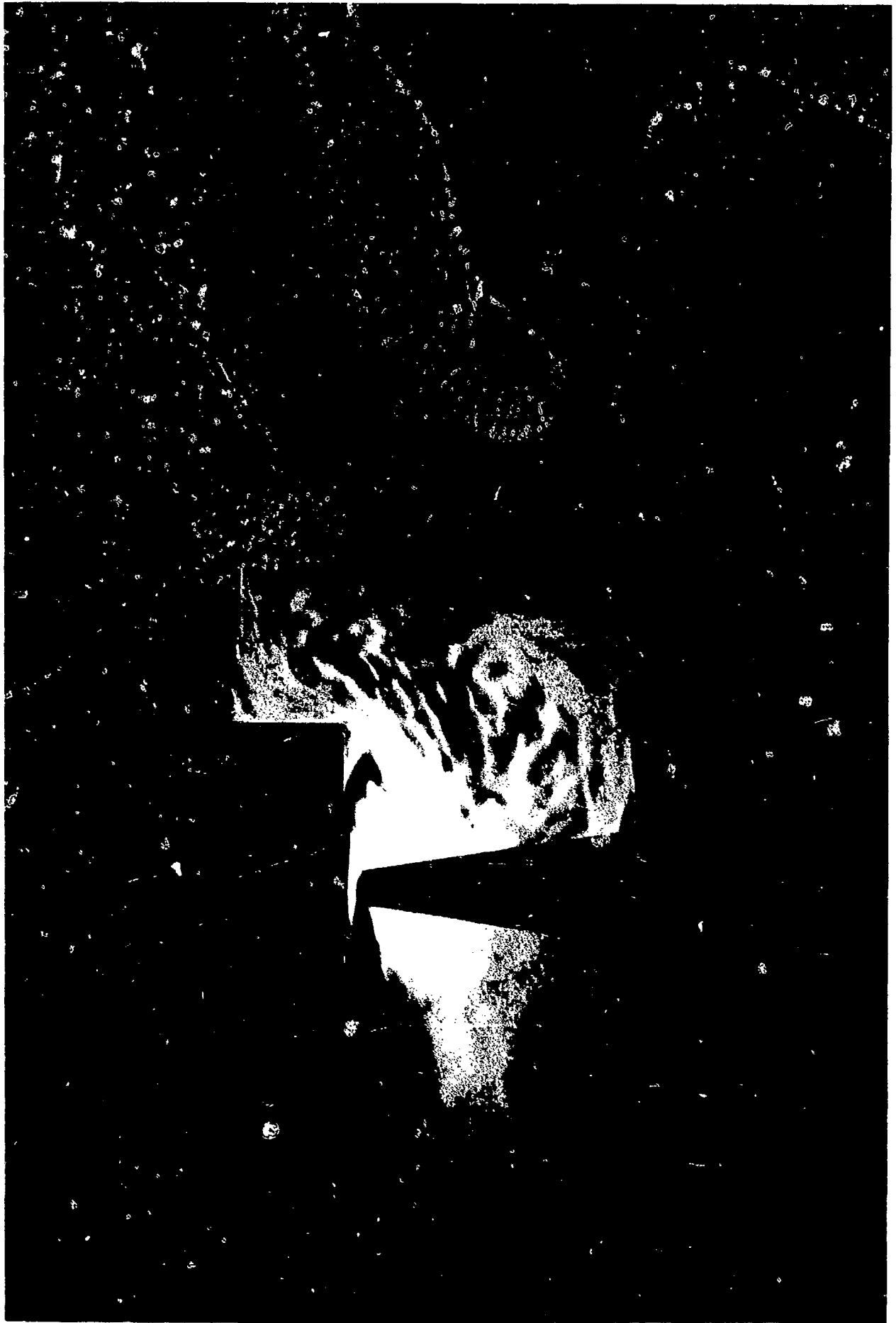
Figure 49. Tapered three-knife stepped seal with flow in the LTSD direction (flow up the step), schlieren flow visualization at low \Delta P .
