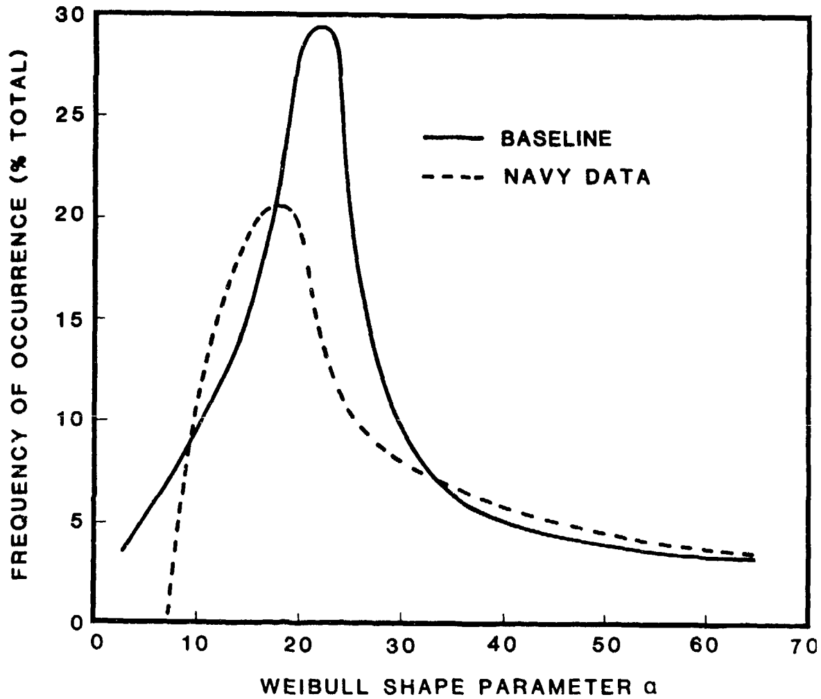
FIGURE 12. COMPARISON OF OVERALL DISTRIBUTION OF SCATTER IN NAVY AND BASELINE STATIC STRENGTH DATA.
