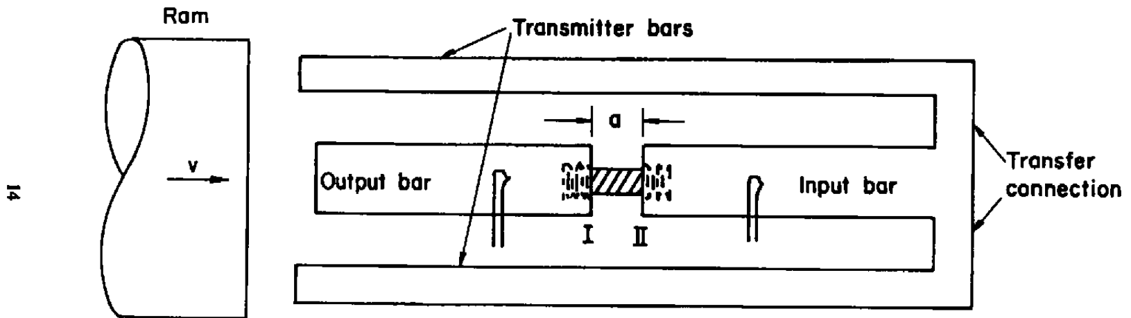
Figure 6. A Possible Configuration for Tension Test.
