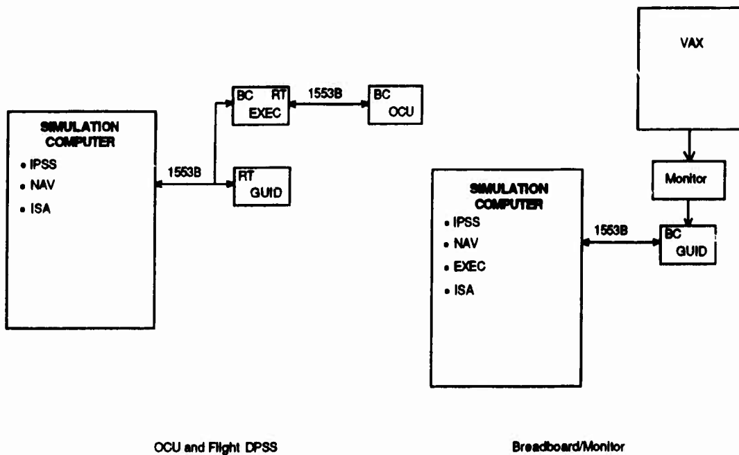
Figure 10. Hardware Configurations
