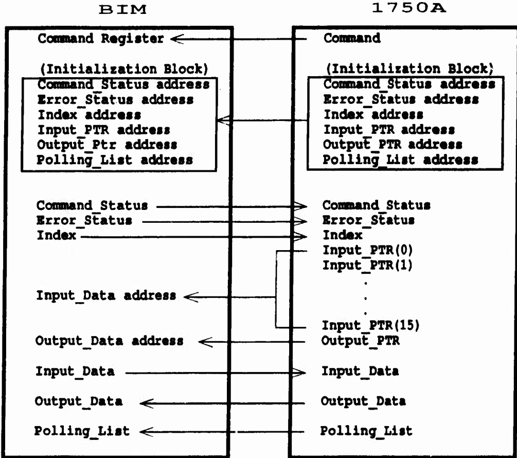
Figure 15. BIM/1750A Interface
