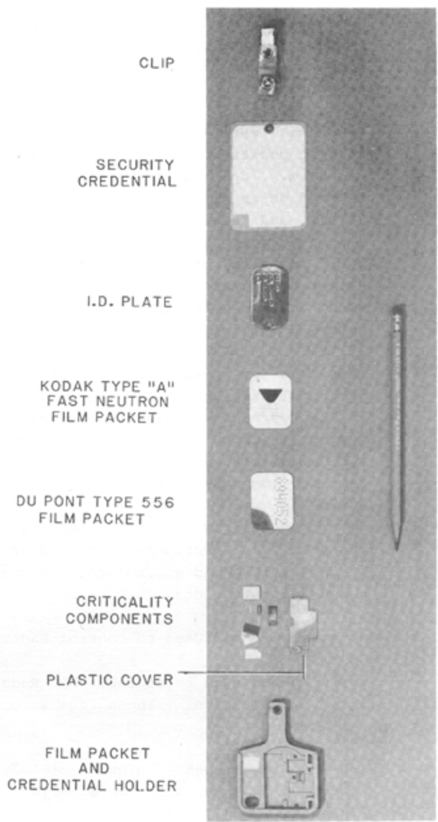
Figure 2.5 NTS combination personnel dosimeter and security credential holder.
