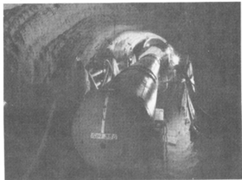
Agabian water tank in E drift after partial stemming pour
