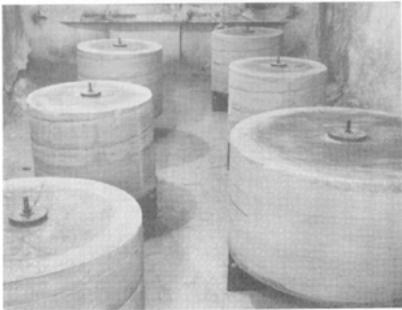
SRI jointed models in D-1 drift
