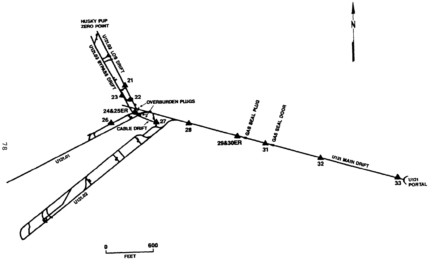
Figure 3.4 HUSKY PUP event - underground RAMS.
