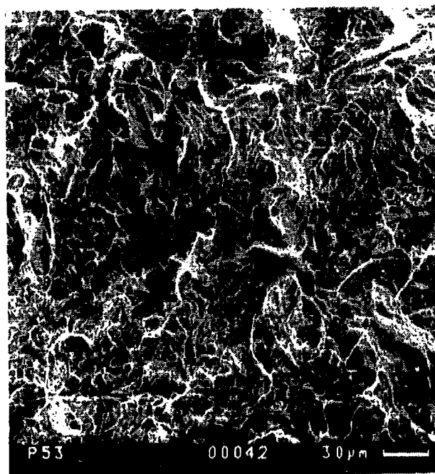
SEM Fractograph, 300 ×
