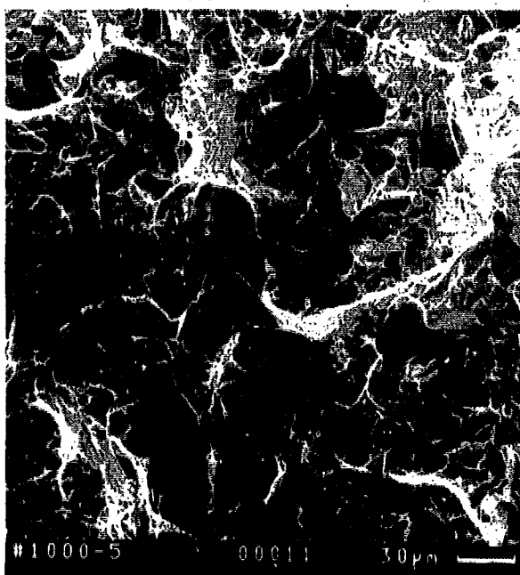
SEM Fractograph, 300 ×
