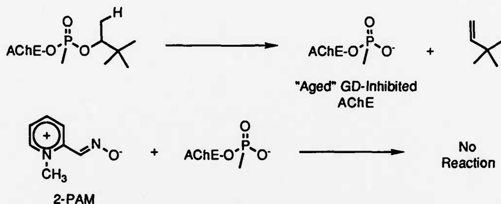
Scheme 4. Aging of GD-inhibited AChE.
