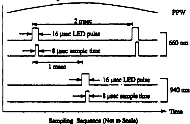
Figure 6. Timing sequence for for sampling and analog to digital conversion of photometric data.
