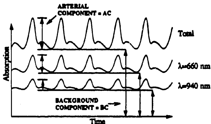
Figure 3. Representative absorption waveforms for SaO_2 measurements (simulated).
