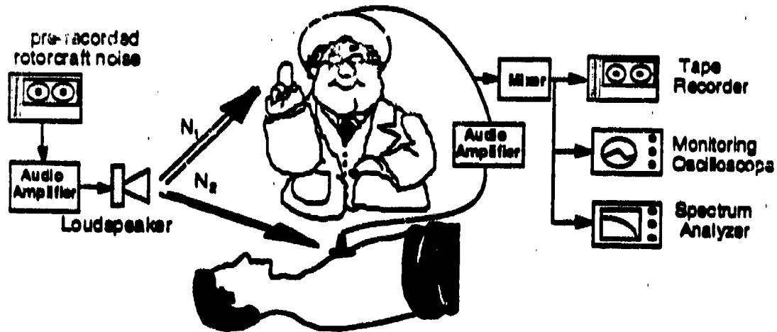
Figure 4.1-4: Psychoacoustic Experiment
