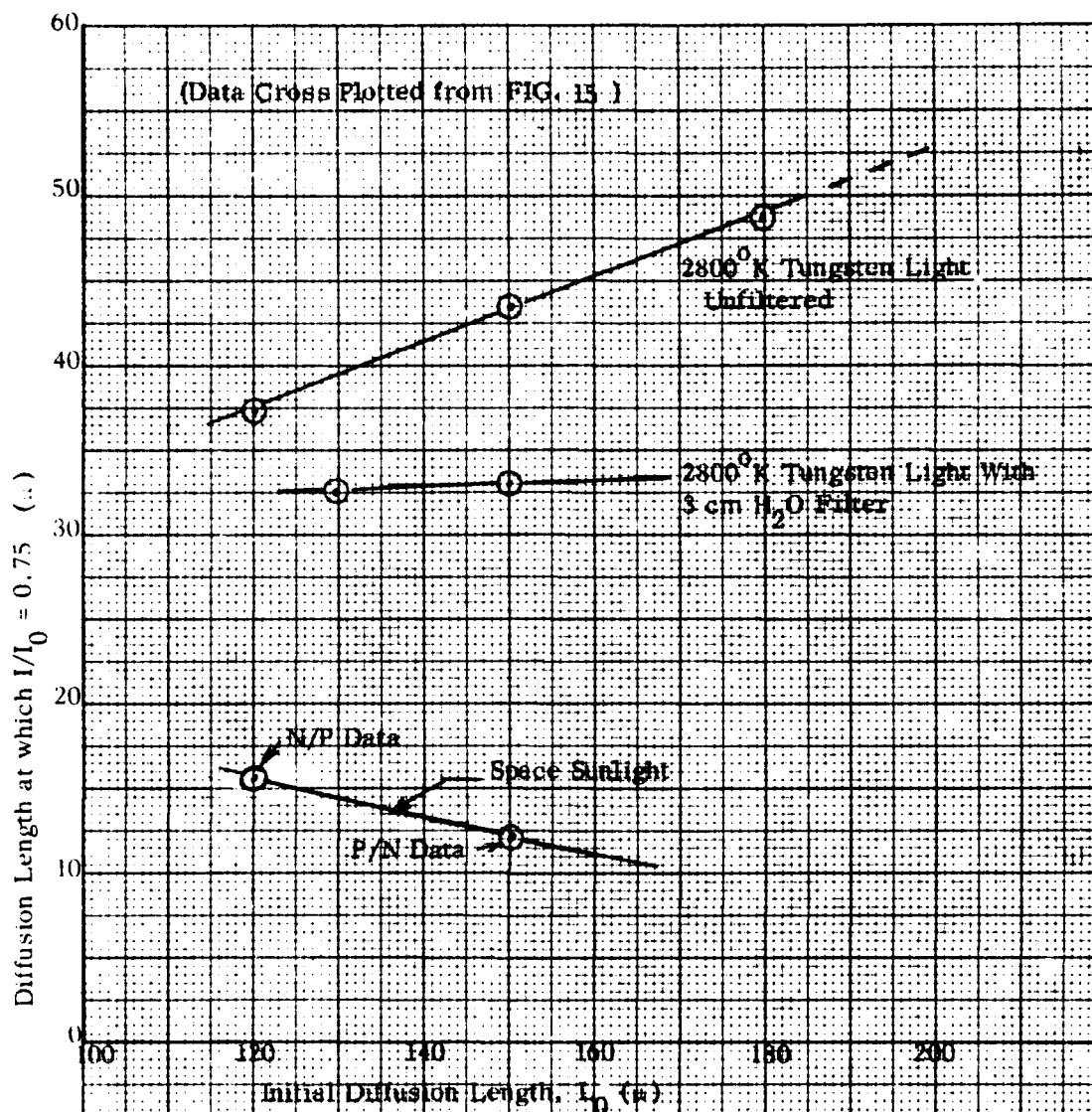
FIG. 16 DEGRADED VS. INITIAL DIFFUSION LENGTH FOR 75% SHORT CIRCUIT CURRENT IN SILICON SOLAR CELLS
