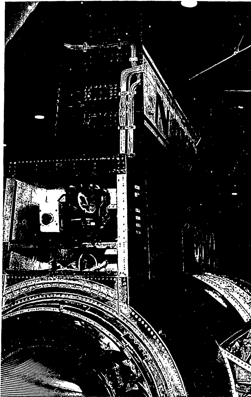
An infrared horizon-scanner, with cover plate removed, is seen here in its compartment behind the upper speed brakes of an X-15 before a research flight to high altitude. The instrument helped measure background noise for the design of satellite instruments. Those bundles of stainless-steel pressure tubes on the aft end of the upper vertical tail lead to pressure rakes on the sides of the tail.
