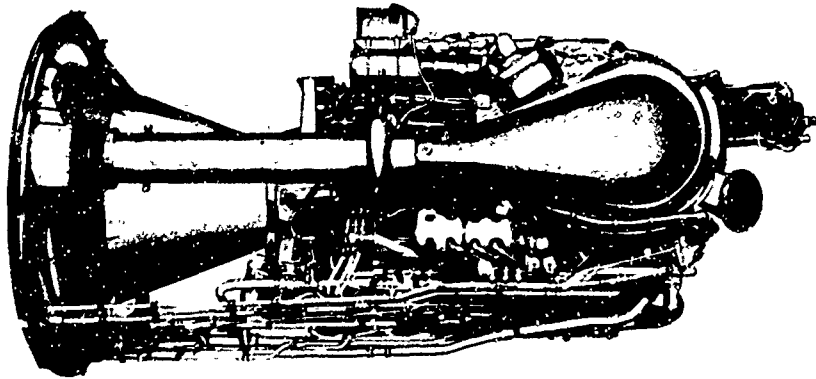
A closeup of the X-15's remarkable XLR-99 rocket engine. Its 57 000-lb. maximum thrust is equivalent at burnout to 600 000 hp. The engine can be throttled from 40-percent to 100-percent thrust. Its propellants flow at the rate of 13 000 lb. per minute at maximum thrust, exhausting the entire 18 000-lb. fuel supply in 85 seconds. The engine's nozzle diameter is 39.3 in.; its over-all length, 82 in.; its weight, 1025 lb.
