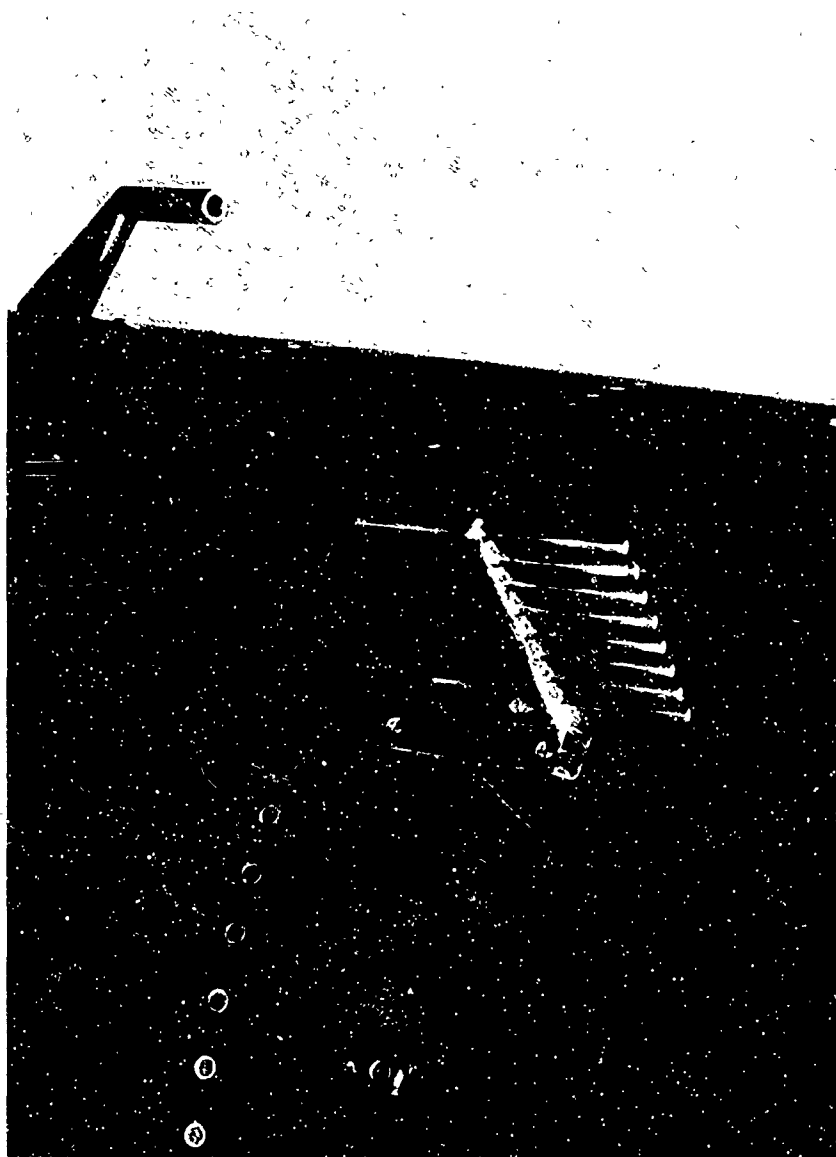
One of the many tools of the X-15's research is this multiple-probe pressure rake, mounted on the forward fuselage to measure boundary-layer airflow at hypersonic speeds. Below the rake is one of the 140 holes cut in the aircraft's skin to measure surface pressures. Above and behind the rake is a pressure probe, used only during landing, for the pilot's airspeed indicator.
