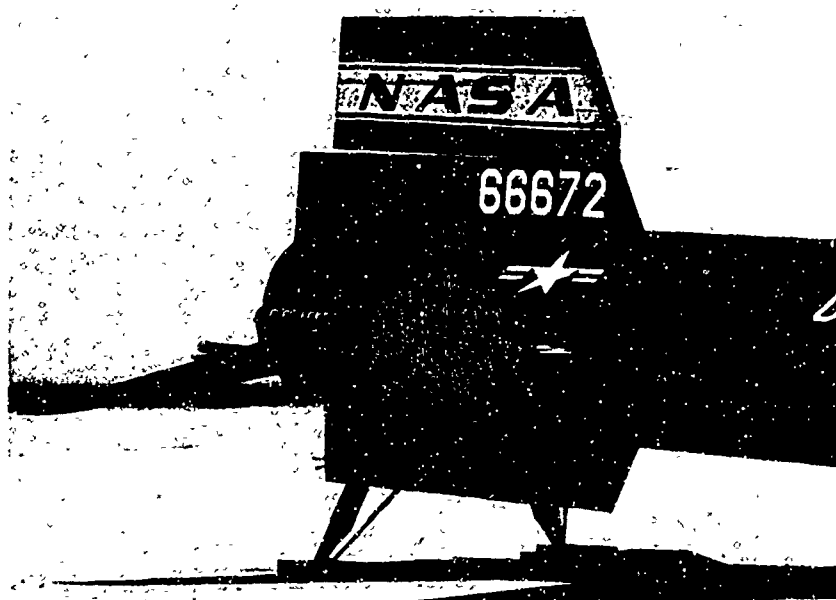
This photograph provides an unusually clear view of the X-15's unique main landing gear, and shows how much of the lower vertical tail is left after its bottom part has been jettisoned for landing. The photo also reveals the new, knife-sharp leading edge that has been given to the X-15-3 configuration's upper vertical tail in order to study heat transfer through 2500-deg. airflow.
