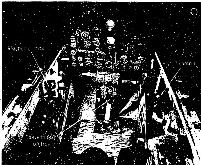
The X-15's cockpit is quite like a jet fighter's, except for its unique arrangement of three control sticks. The one at left governs the jet reaction controls, in space-equivalent flight. The one at right is used in high-G flight and is mechanically linked to the conventional stick at center.
