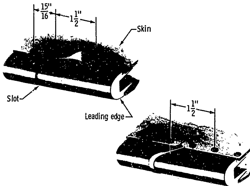
Top drawing shows a typical buckle in the wing skin of the X-15, caused by uneven expansion between the leading edge and the area directly behind it in hot airflow at hypersonic speed. Bottom drawing shows how covering the slots with small Inconel tabs and adding a rivet prevented recurrence of the buckling.
