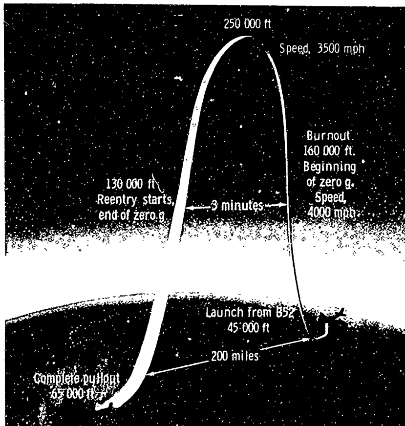
Profile and pertinent details of a flight in which the X-15 achieved its design goals in speed and altitude and came very close to that point in structural temperature.
