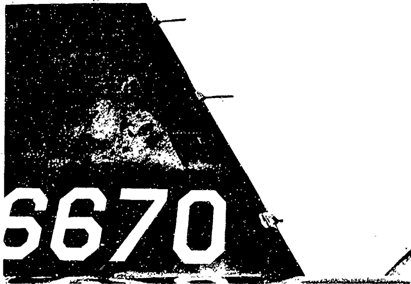
Pressure tubes in the leading edge of the X-15's upper vertical tail measure airflow conditions in the wake of the fuselage. The craft's instrumentation, elaborate despite weight and volume restrictions, measured pressure at 160 locations.
