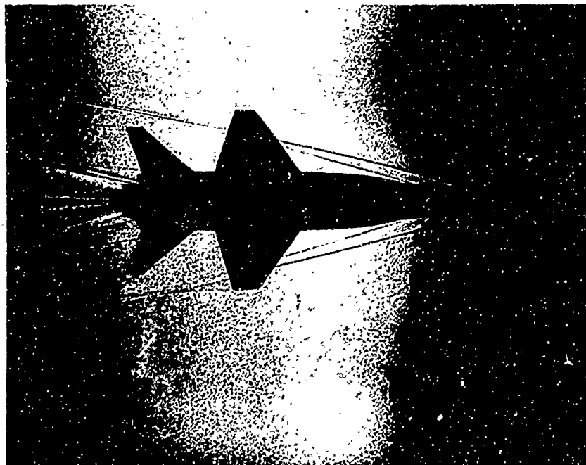
These dramatic photographs of free-flight models of the X-15 being fired into a wind tunnel vividly detail the shock-wave patterns for airflow at Mach 3.5 (above) and at Mach 6.
