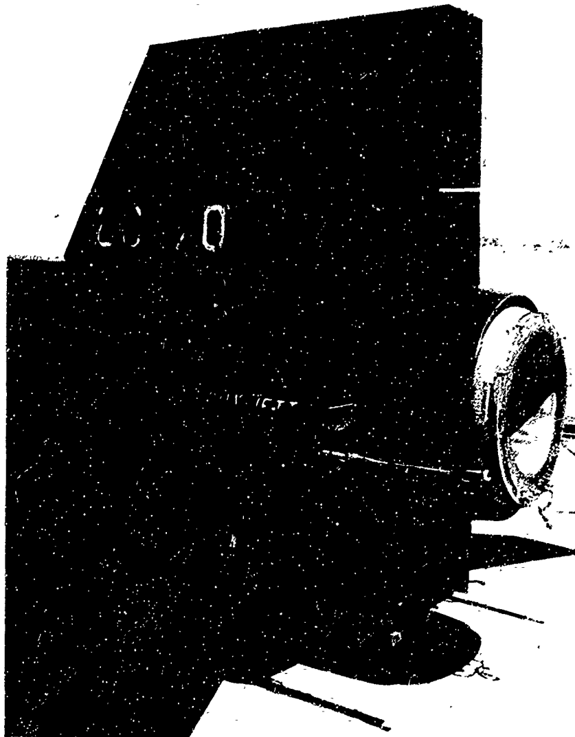
The blunt aft ends of the X-15's side fairings, vertical tails, and the rocket-engine nozzle represent one of the many compromises that a hypersonic configuration demanded. Together they produce as much drag as an F-104 jet fighter.
