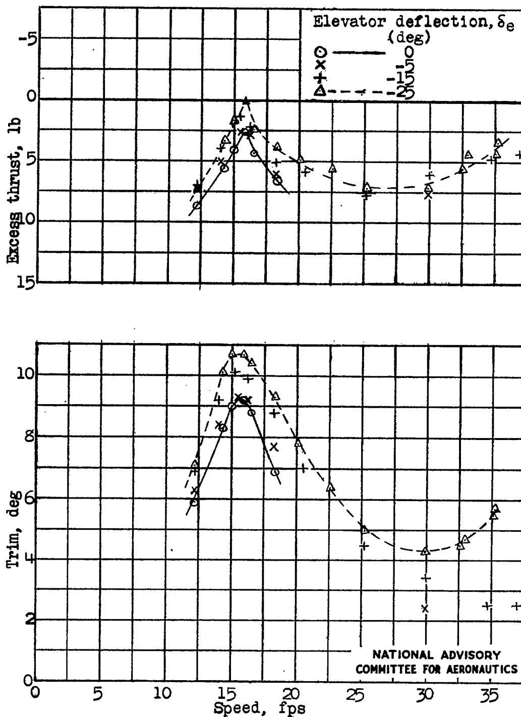
Figure 19.- Model 180-1. Variation of excess thrust and trim with speed. Gross load, 94.3 pounds (165,000 lb, full size); \delta_f = 30^\circ ; center of gravity, 28 percent mean aerodynamic chord.
