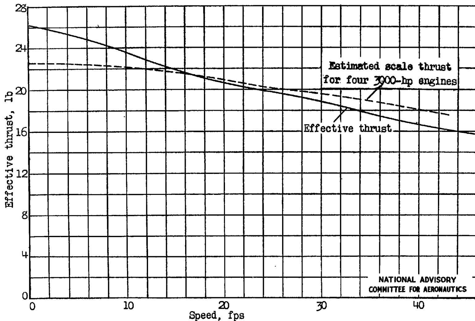
Figure 6.- Model 180. Variation of effective thrust with speed. Trim, 0^\circ ; \delta_f = 30^\circ ; \delta_e = 0^\circ .
