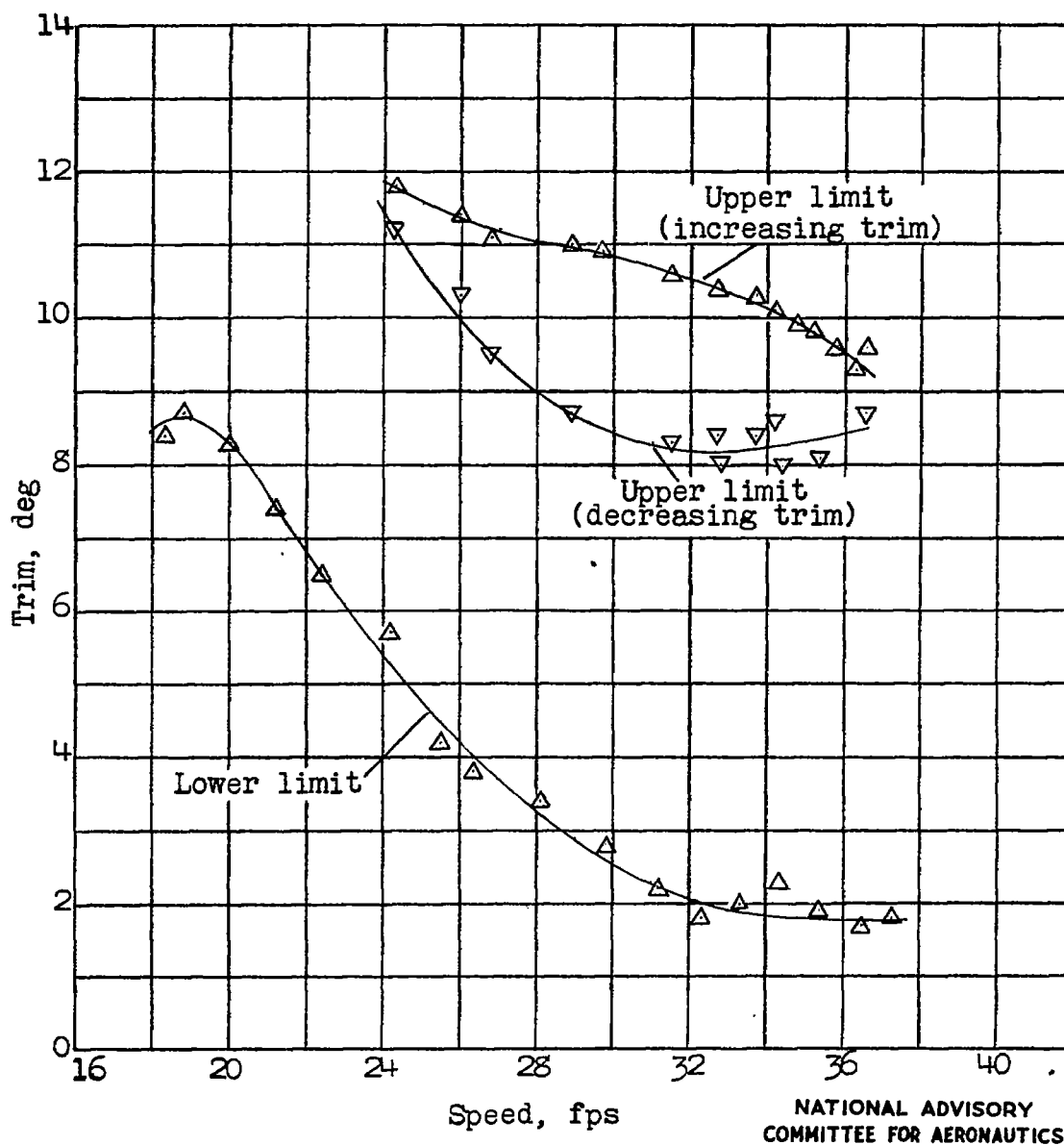
Figure 13.- Model 180-1. Trim limits of stability with power. Gross load, 105.7 pounds (185,000 lb, full size); \delta_f = 30^\circ .
