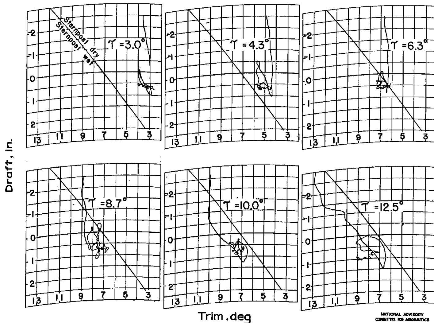
Figure 11. - Model 180-I. Variation of trim and draft during landing. Gross load, 105.7 pounds (185,000 lb, full size); center of gravity, 40 percent mean aerodynamic chord; without power; \delta_f = 55^\circ .
