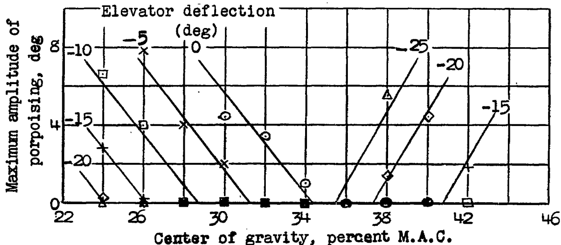
Figure 16.- Model 180-1. Maximum amplitude of porpoising at different positions of the center of gravity with power. Gross load, 105.7 pounds (185,000 lb, full size); \delta_f = 30^\circ . NATIONAL ADVISORY COMMITTEE FOR AERONAUTICS
