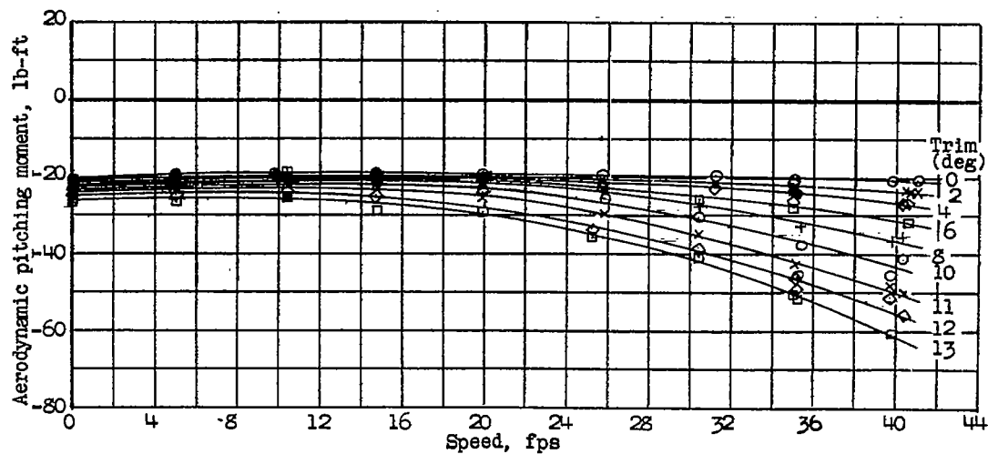
Figure 7.- Model 180. Variation of aerodynamic lift and pitching moments with trim. \delta_f = 30^\circ ; center of gravity, 24 percent mean aerodynamic chord; full power.
