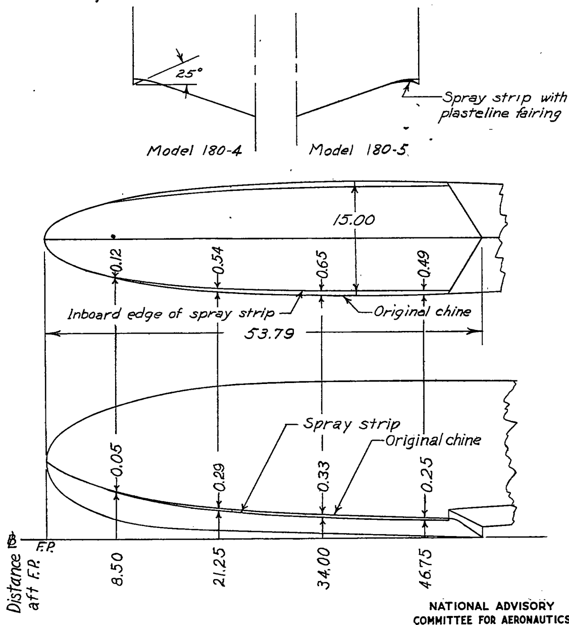
Figure 24.- Langley tank models 180-4 and 180-5. Spray strips on forebody. (Dimensions are in in.)
