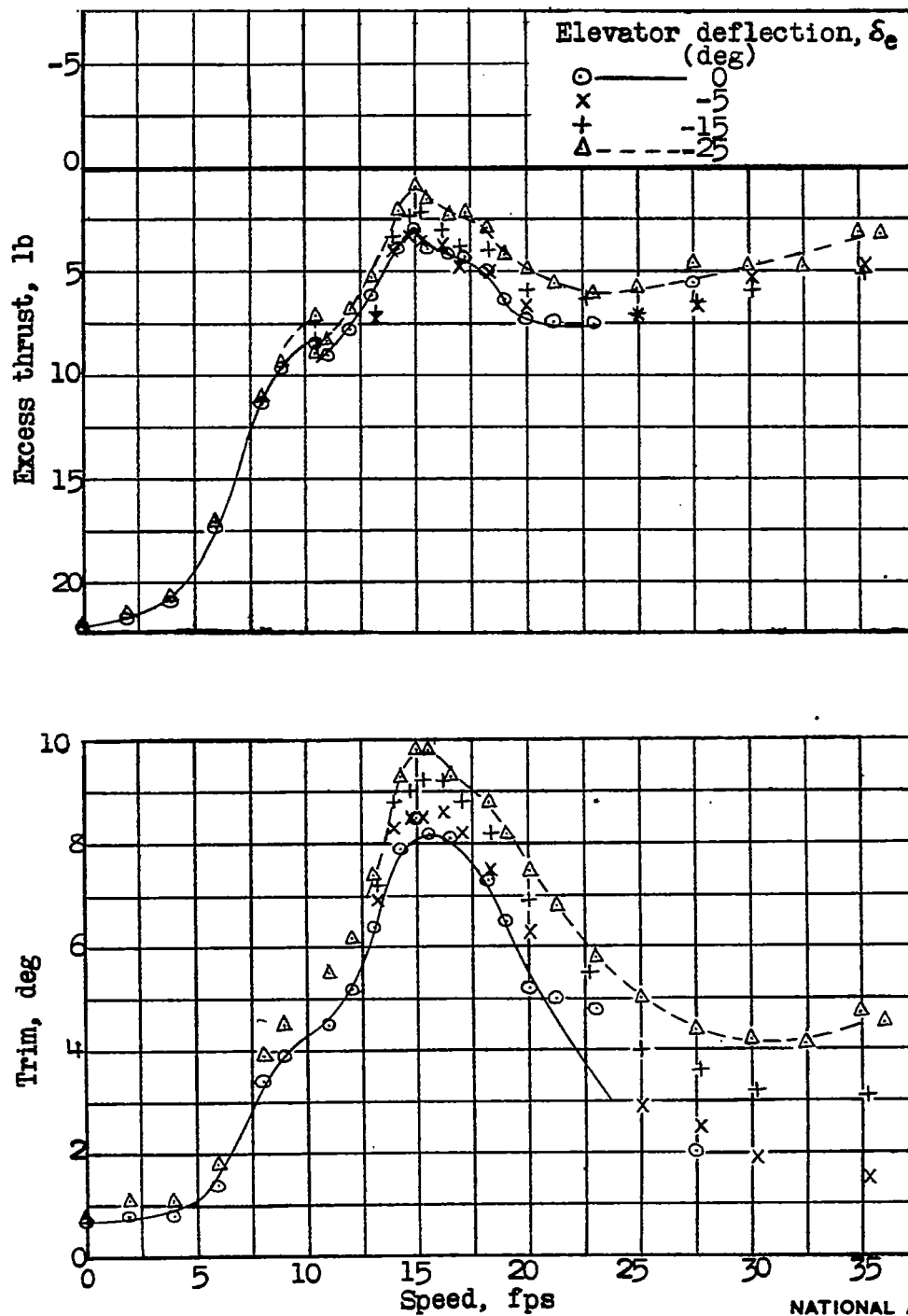
Figure 18.- Model 180. Variation of excess thrust and trim with speed. Gross load, 94.3 pounds (165,000 lb, full size); \delta_f = 30^\circ ; center of gravity, 28 percent mean aerodynamic chord.
