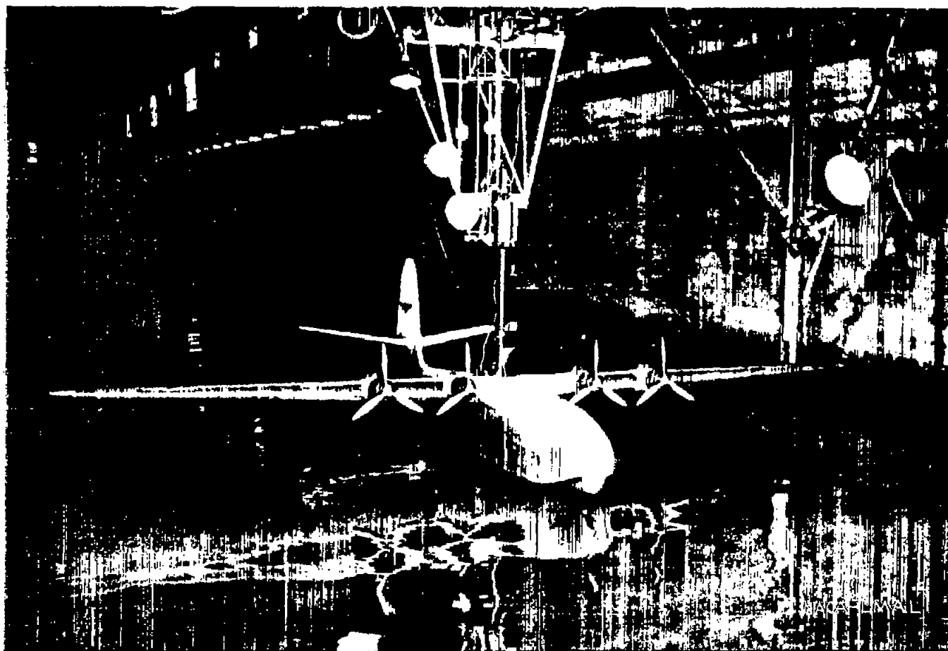
Figure 5.- Model 180 and towing apparatus.
