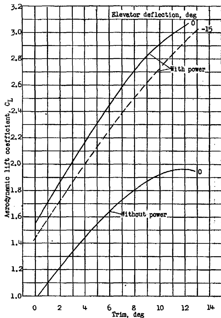
Figure 8.- Model 180. Variation of aerodynamic lift and pitching-moment coefficients with trim. \delta_f = 30^\circ ; center of gravity, 24 percent mean aerodynamic chord; V = 35 feet per second.
