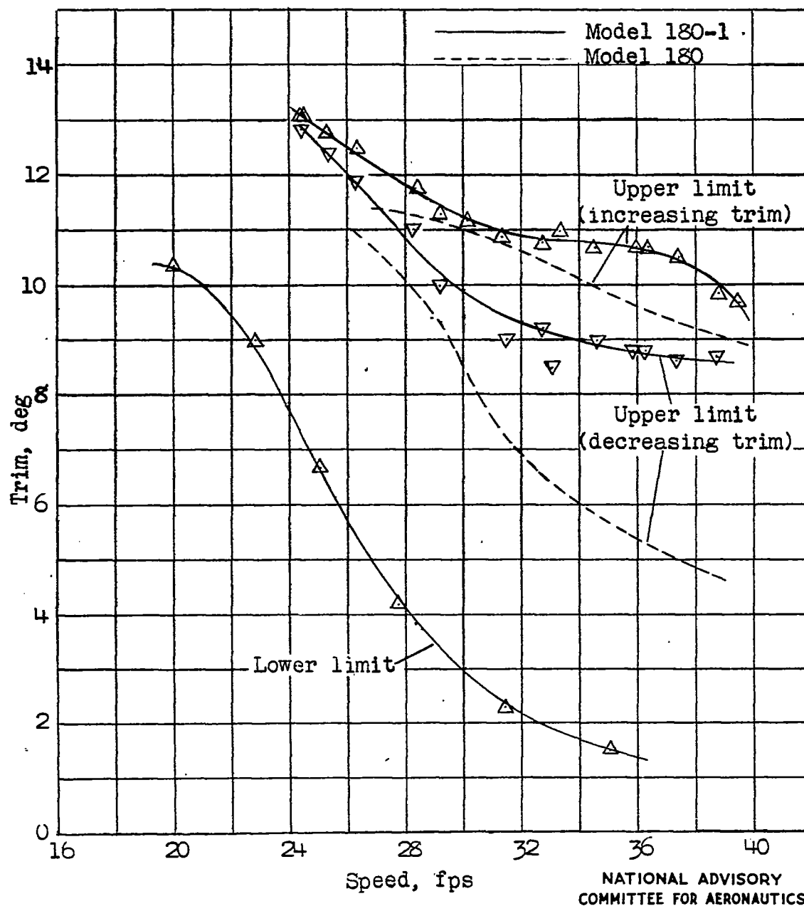
Figure 12.- Models 180 and 180-1. Trim limits of stability without power. Gross load, 94.3 pounds (165,000 lb, full size); \delta_f = 55^\circ .
