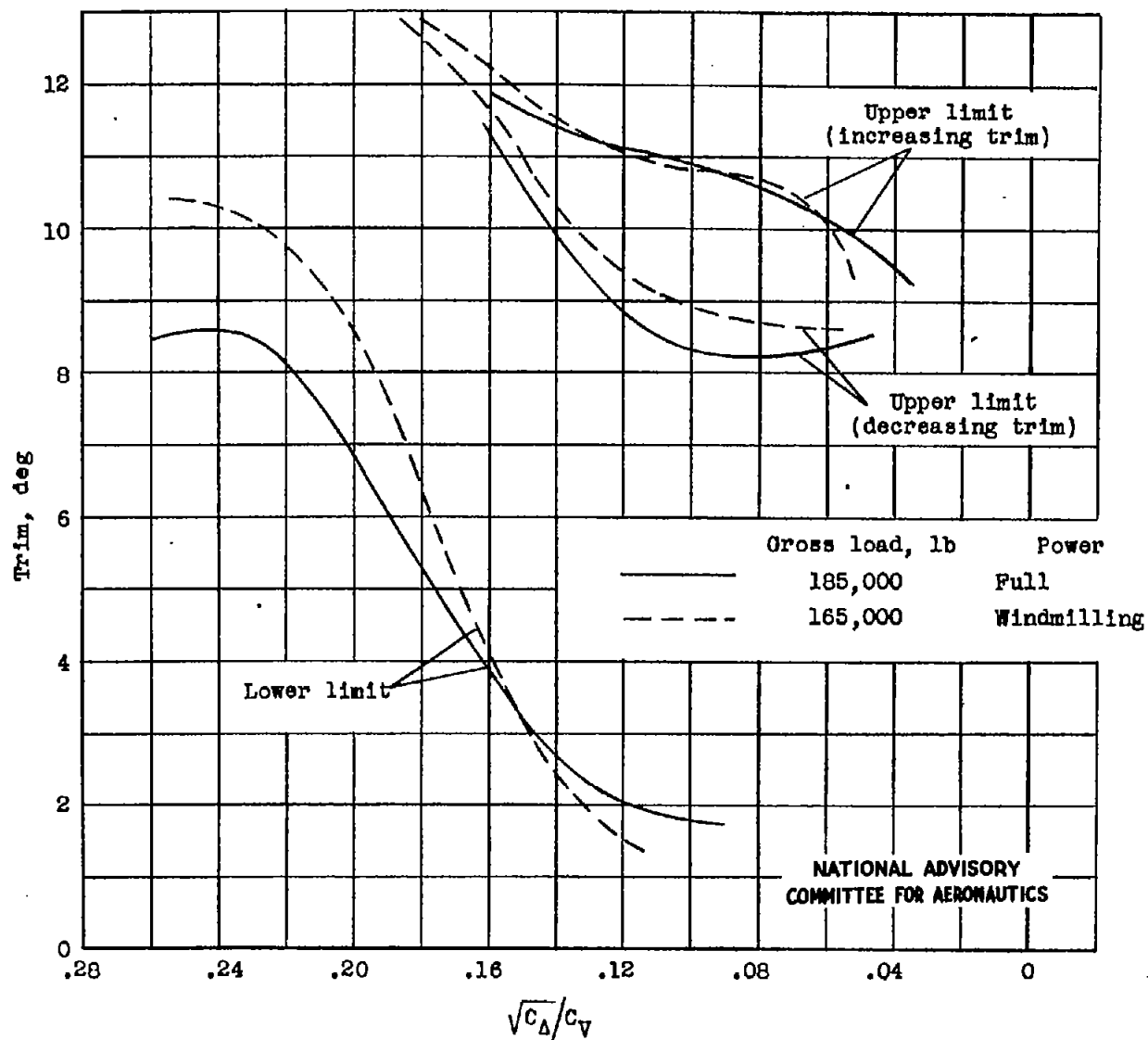
Figure 14.- Model 180-1. Nondimensional trim limits of stability.
