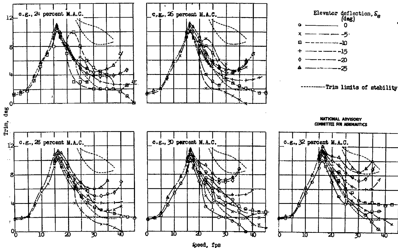
Figure 15.- Model 180-1. Variation of trim with speed. Gross load, 105.7 pounds (185,000 lb, full size); \delta_T = 30^\circ ; full power.
