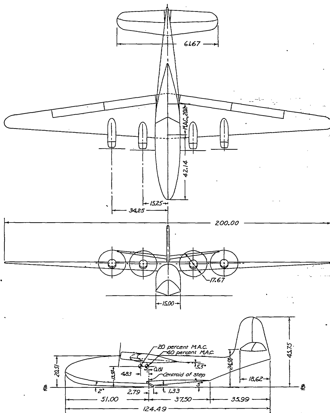
Figure 2.-Langley tank model 180. General arrangement. (Dimensions in in.)
