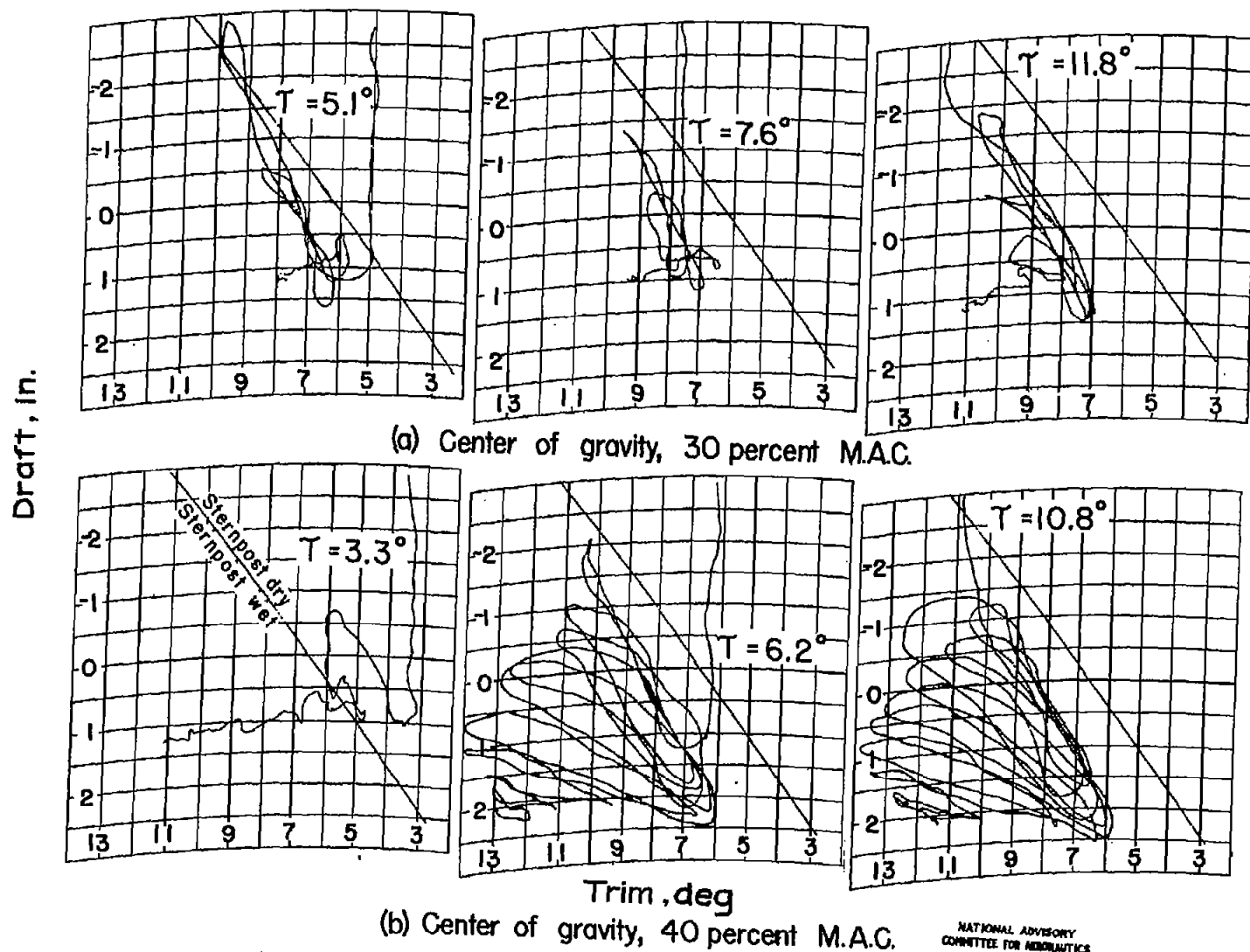
Figure 9.- Model 180. Variation of trim and draft during landing. Gross load, 94.3 pounds (165,000 lb, full size); without power; \delta_f = 55^\circ .
