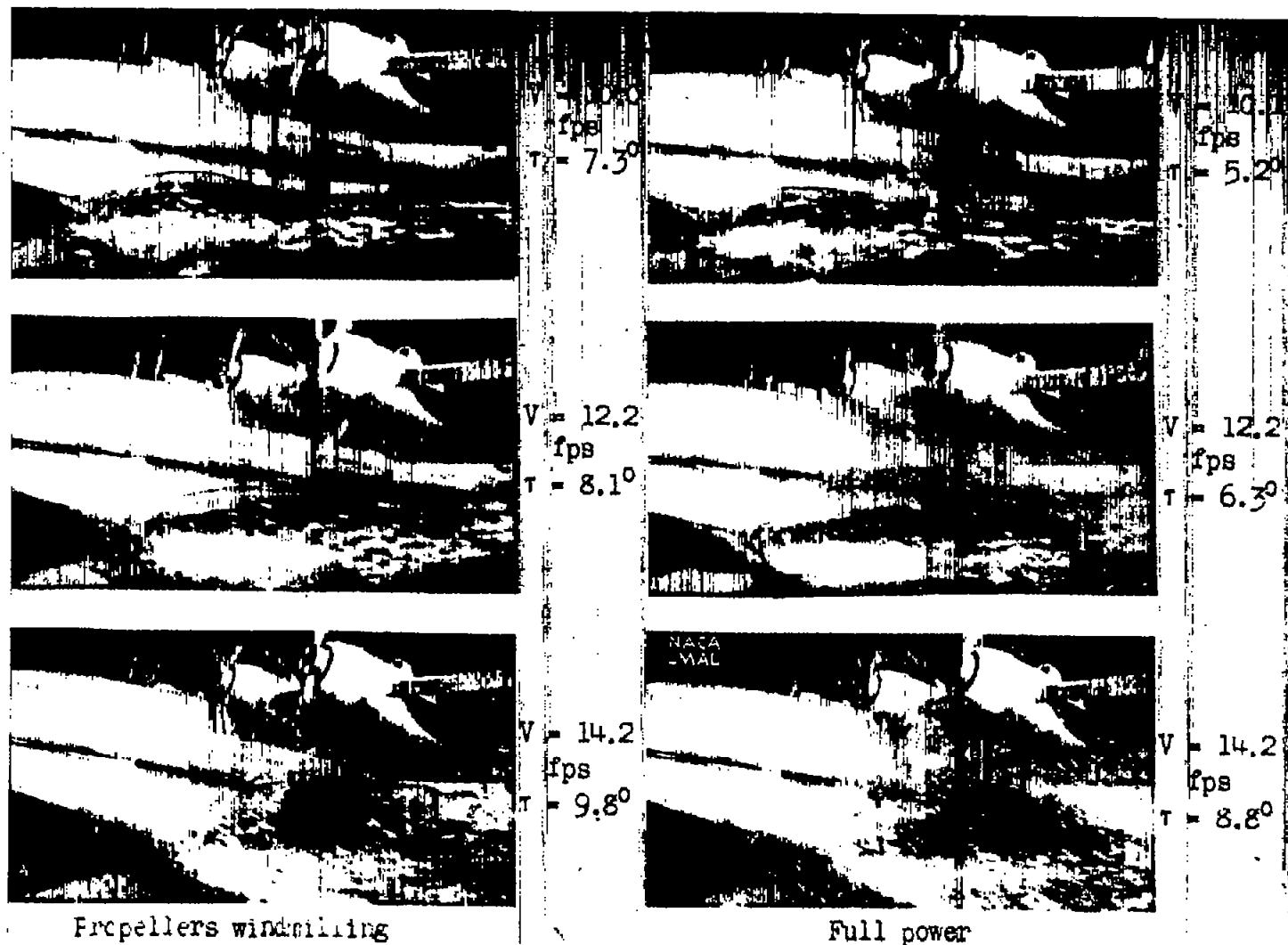
Figure 20.- Concluded. (b) Gross load, 105.7 pounds (135,000 lb, full size)
