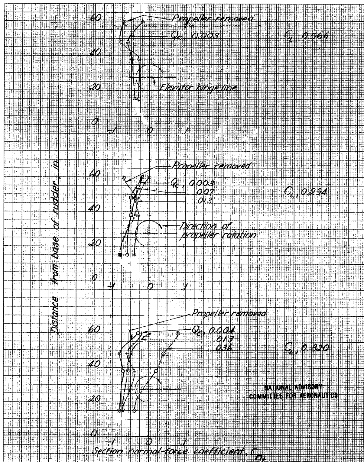
Figure 12.- Spanwise distribution of normal-force coefficient on vertical tail surface. \psi, 0^\circ .
