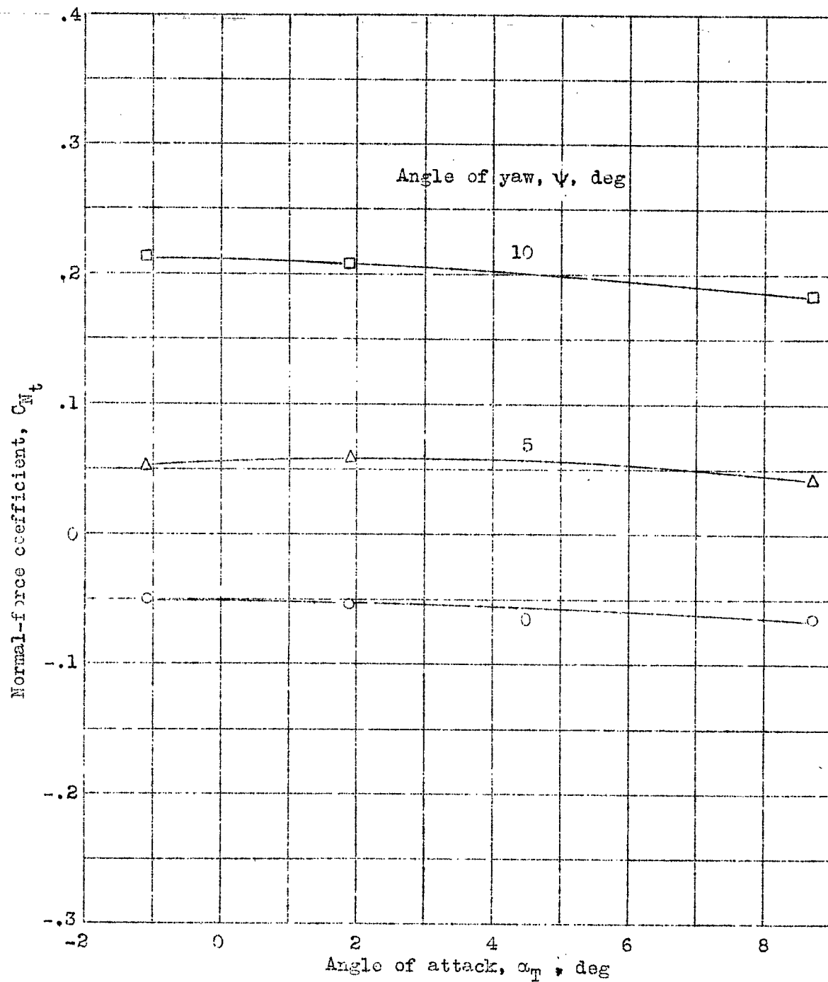
Figure 16.-- Variation of vertical-tail normal-force coefficient with angle of attack. Propeller removed.
