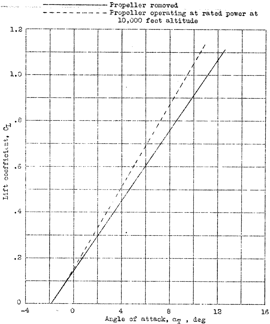
Figure 6.— Lift curves for the P-40K airplane with the propeller removed and operating at rated power at 10,000 feet altitude. Flaps retracted; i_t , 2.0^\circ .
