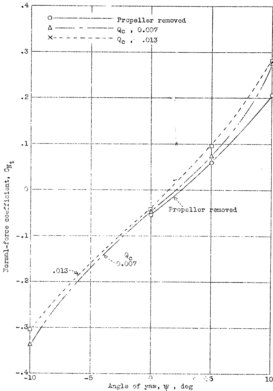
Figure 17.- Effect of propeller operation on the variation of vertical-tail normal-force coefficient with angle of yaw. C_L , 0.294.
