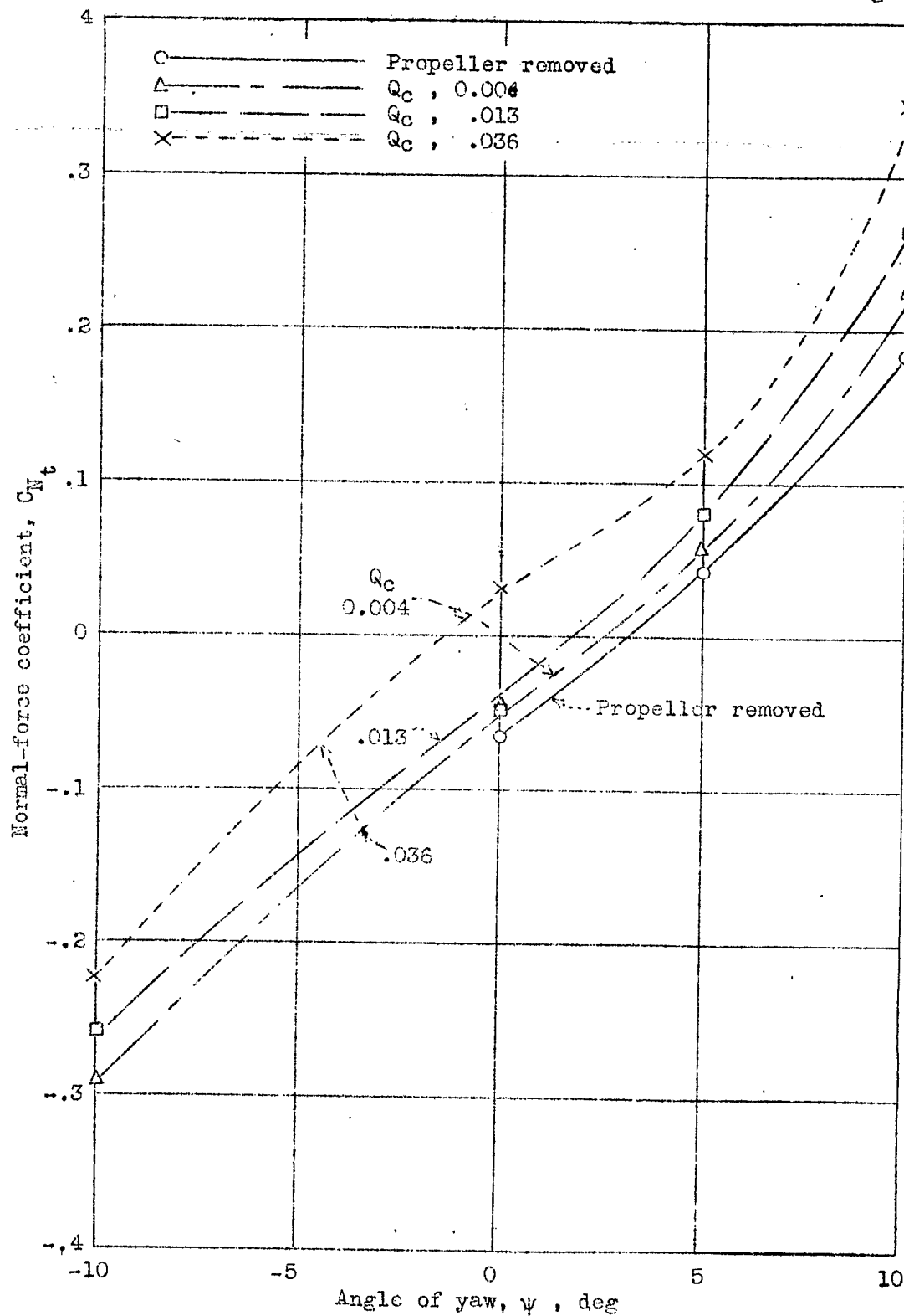
Figure 18.— Effect of propeller operation on the variation of vertical-tail normal-force coefficient with angle of yaw. C_{I_1} : 0.820.
