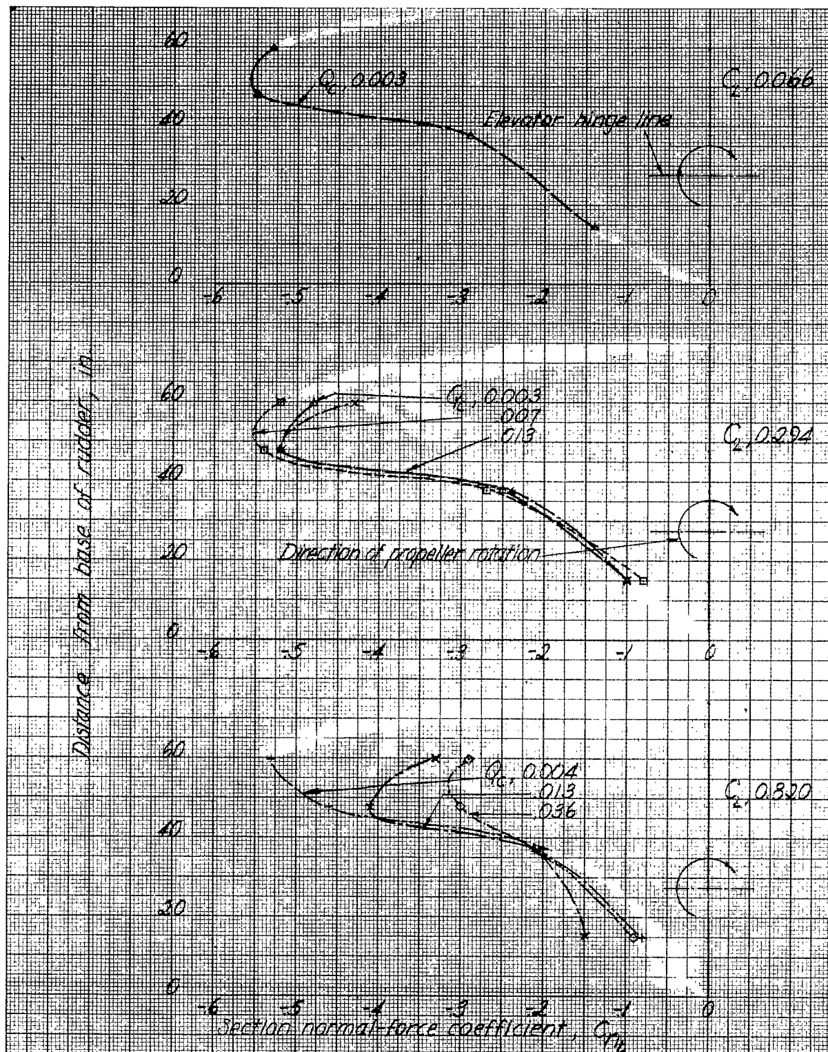
Figure 15.- Spanwise distribution of normal-force coefficient on vertical tail surface. \psi , -10^\circ .
