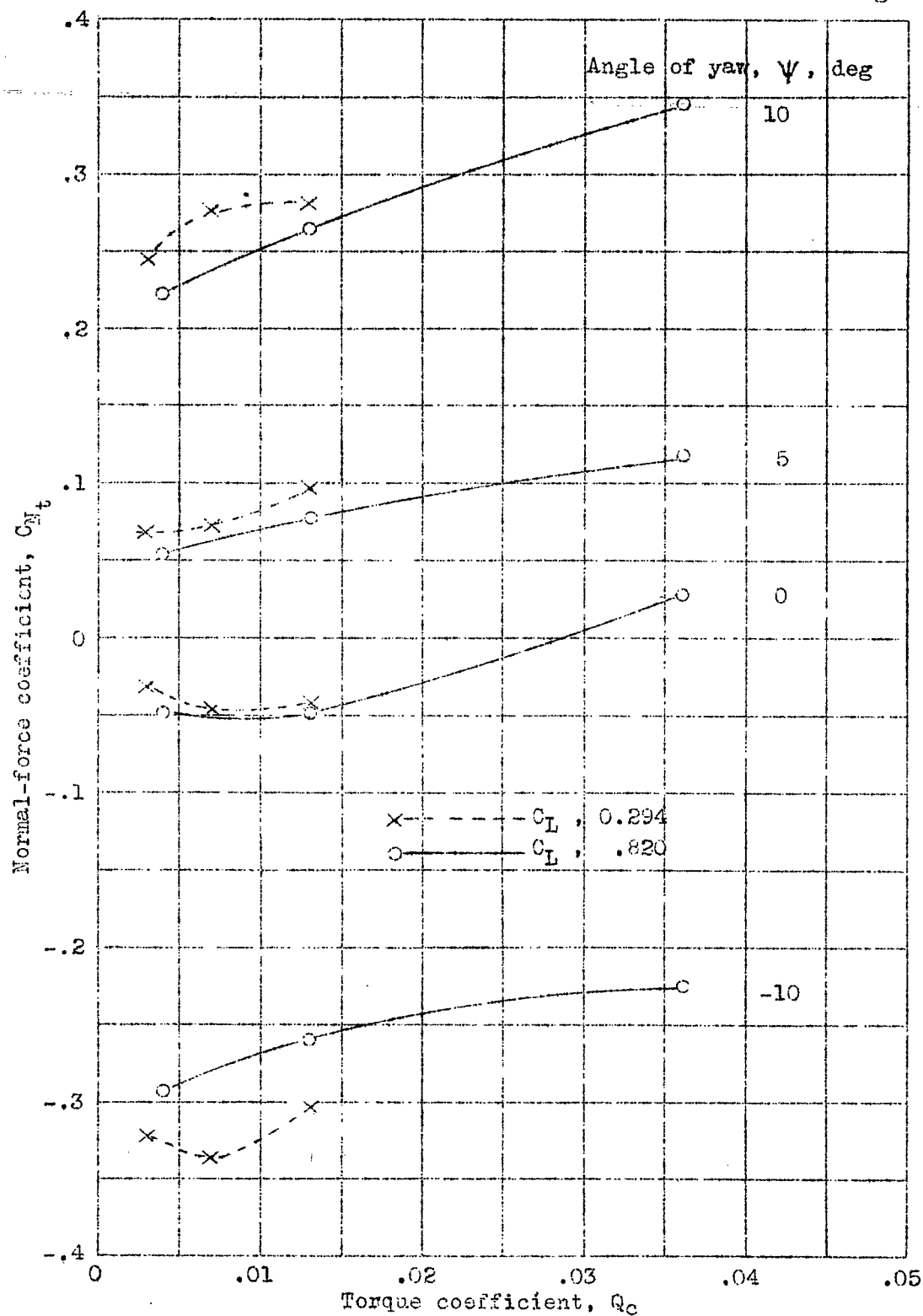
Figure 19.- Effect of slipstream rotation on the vertical-tail normal-force coefficient.
