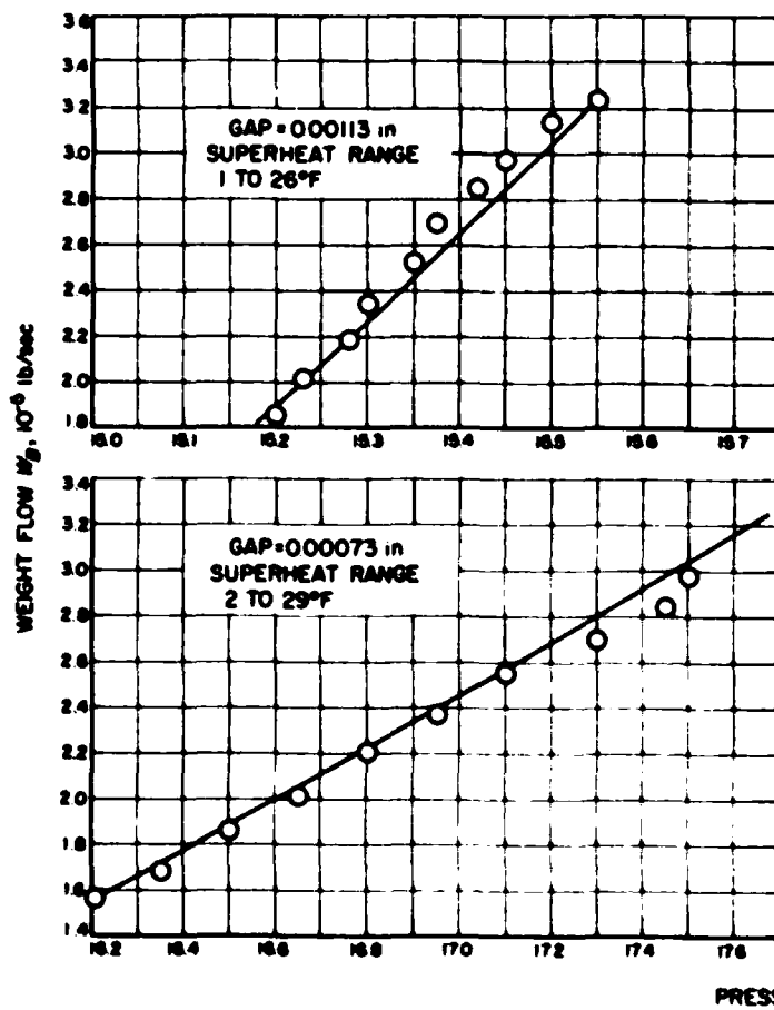
Figure 21. Weight flow through bearing vs absolute pressure at bearing entrance
