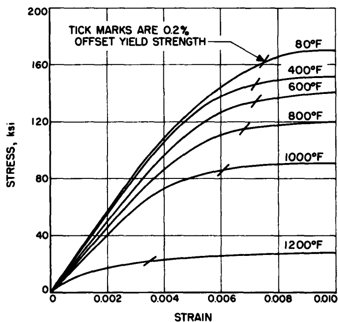
Figure 109. Typical stress-strain curves for 17-7 PH (1050) stainless steel
