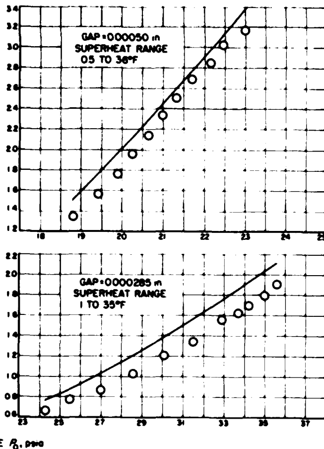
Figure 21. Weight flow through bearing vs absolute pressure at bearing entrance
