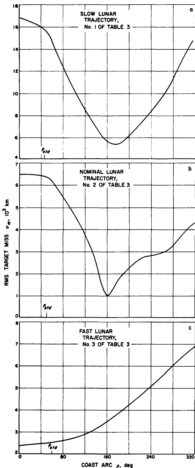
Figure 6. Moon miss distances vs coasting arc
