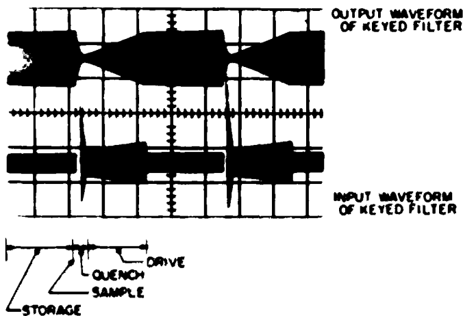
Figure 74. Keyed filter input and output waveforms
