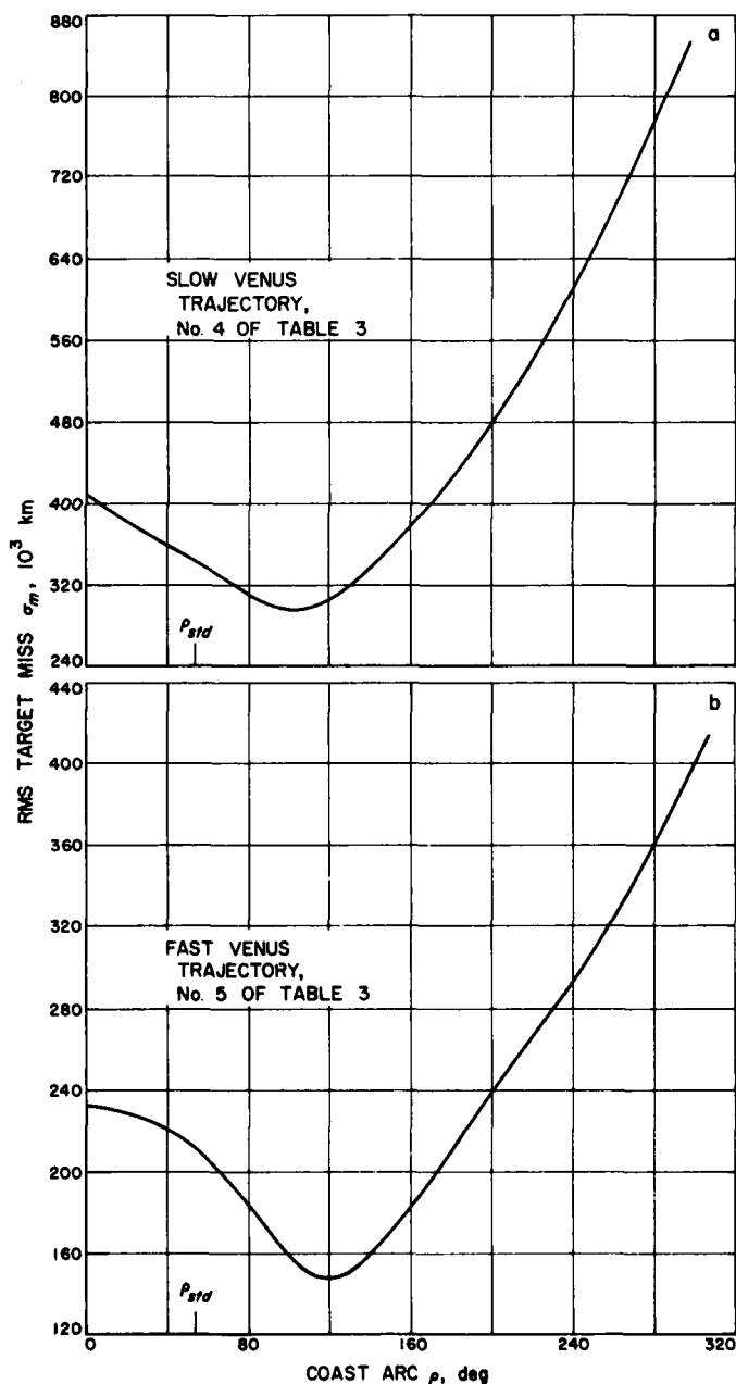
Figure 7. Venus miss distances vs coasting arc
