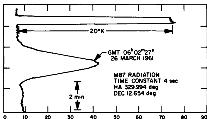
Figure 36. Drift curve of 2388-mc radiation for M87
