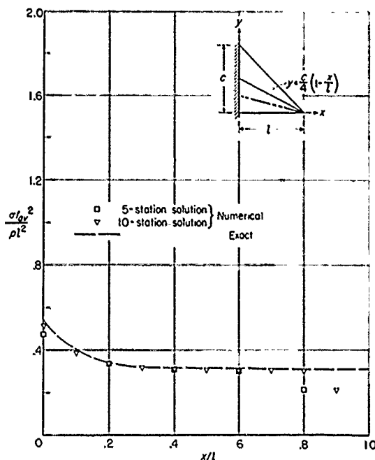
FIGURE 11.—Numerical and exact solutions of the differential equations (obtained by assuming linear chordwise deflections) for the maximum principal stress along the line y = \frac{c}{4}(1 - \frac{x}{l}) of a 45^\circ delta plate of symmetrical double-wedge airfoil section and constant thickness ratio under uniform load.
