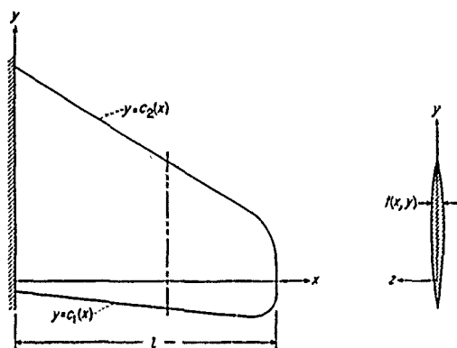
FIGURE 1.—Coordinate system used in the present analysis for a cantilever plate of arbitrary shape with arbitrary thickness variation.
