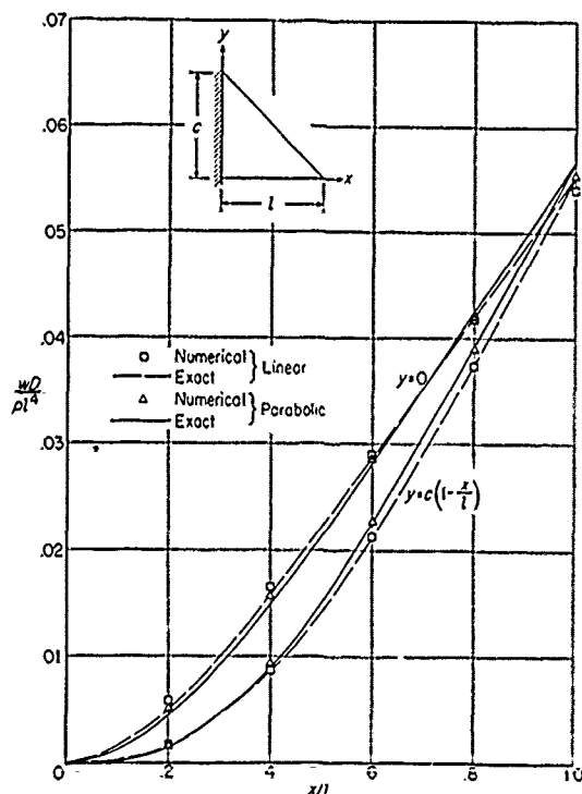
FIGURE 8. Numerical and exact solutions of the differential equations for the deflections of the free edges of a 45^\circ delta plate of uniform thickness under uniform load.
