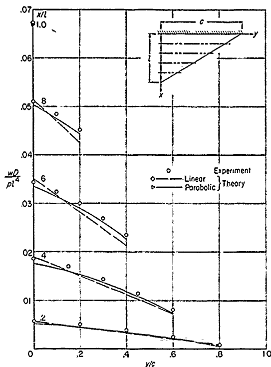
FIGURE 3.—Deflections of a 60° delta plate of uniform thickness under uniform load.
