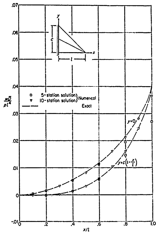
FIGURE 10.—Numerical and exact solutions of the differential equations (obtained by assuming linear chordwise deflections) for the deflections along the free edges of a 45^\circ delta plate of symmetrical double-wedge airfoil section and constant thickness ratio under uniform load
