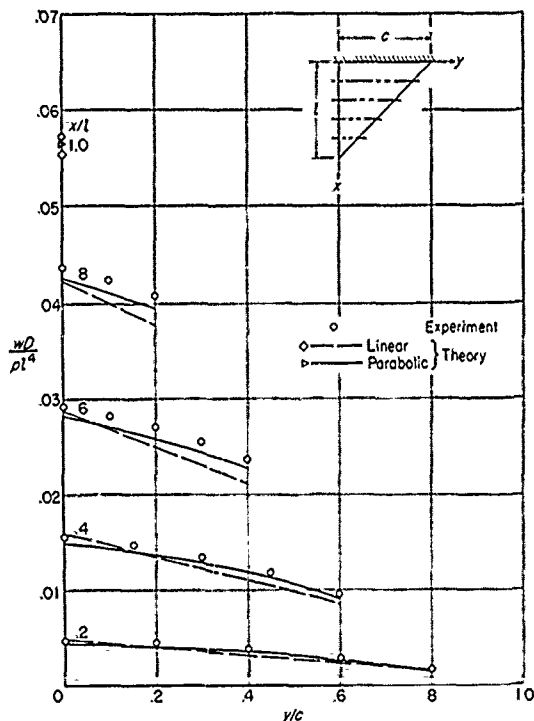
FIGURE 2.—Deflections of a 45° delta plate of uniform thickness under uniform load.
