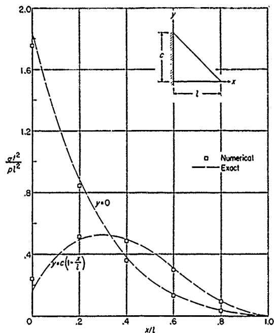
FIGURE 9.—Numerical and exact solutions of the differential equations (obtained by assuming linear chordwise deflections) for the maximum principal stresses along the free edges of a 45^\circ delta plate of uniform thickness under uniform load.
