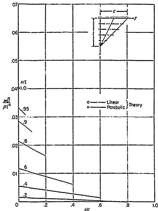
FIGURE 4.—Deflections of a 45° delta plate of symmetrical double-wedge airfoil section and constant thickness ratio under uniform load. \bar{D} = \frac{El_s^3}{12(1-\mu^2)}
