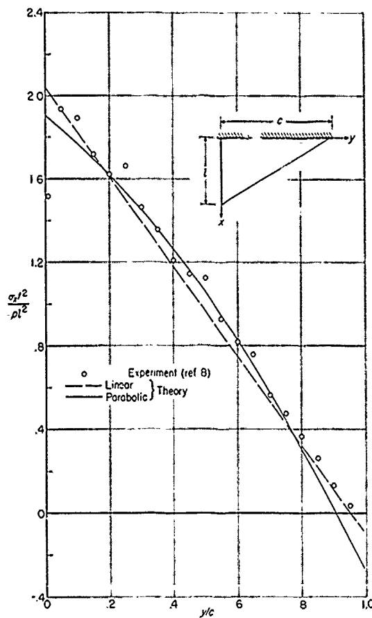
FIGURE 6.—Normal-stress distribution near the root (at \frac{x}{l}=0.0087 ) of a 60° delta plate of uniform thickness under uniform load.
