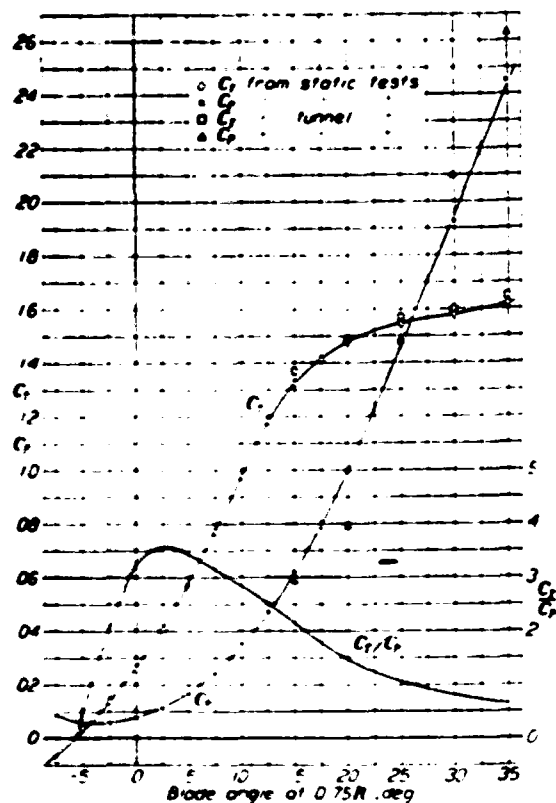
FIGURE 22. Characteristics of 2-blade propeller. The 2-blade propeller C. The 2-blade propeller C.
