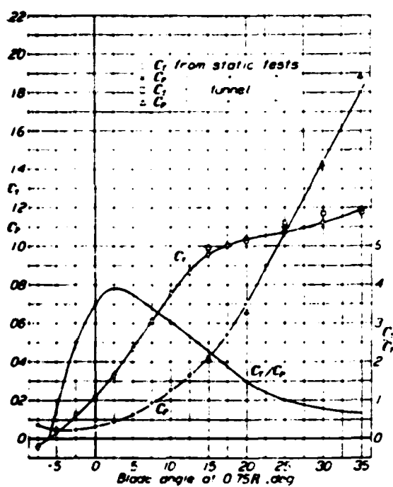
FIGURE 21. Characteristics of 2-blade propeller. The 2-blade propeller C. The 2-blade propeller C.
