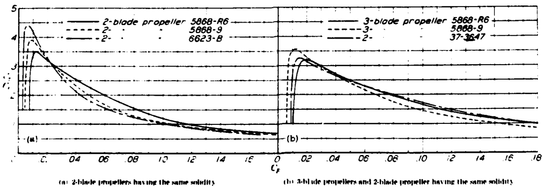
FIGURE 29.- Comparison of propeller characteristics. C_T/C_P against C_P ; V \propto D, 0; M, 0.5 .
