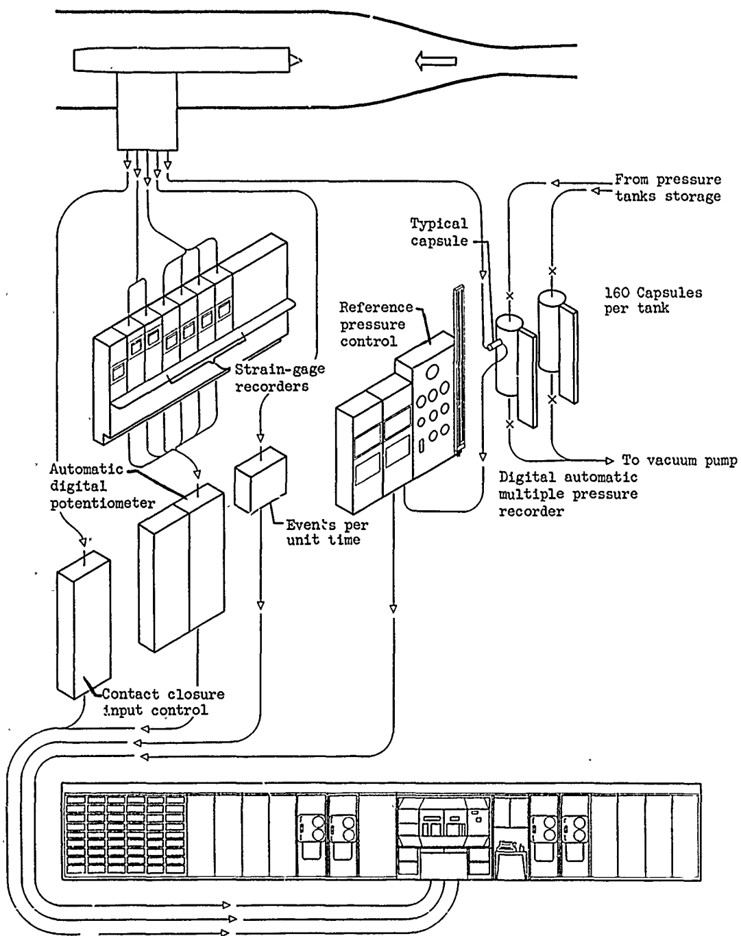
Figure 11. - Wind-tunnel equipment; automatic data recording and processing system, Lewis 8- by 6-foot Supersonic Wind Tunnel.
