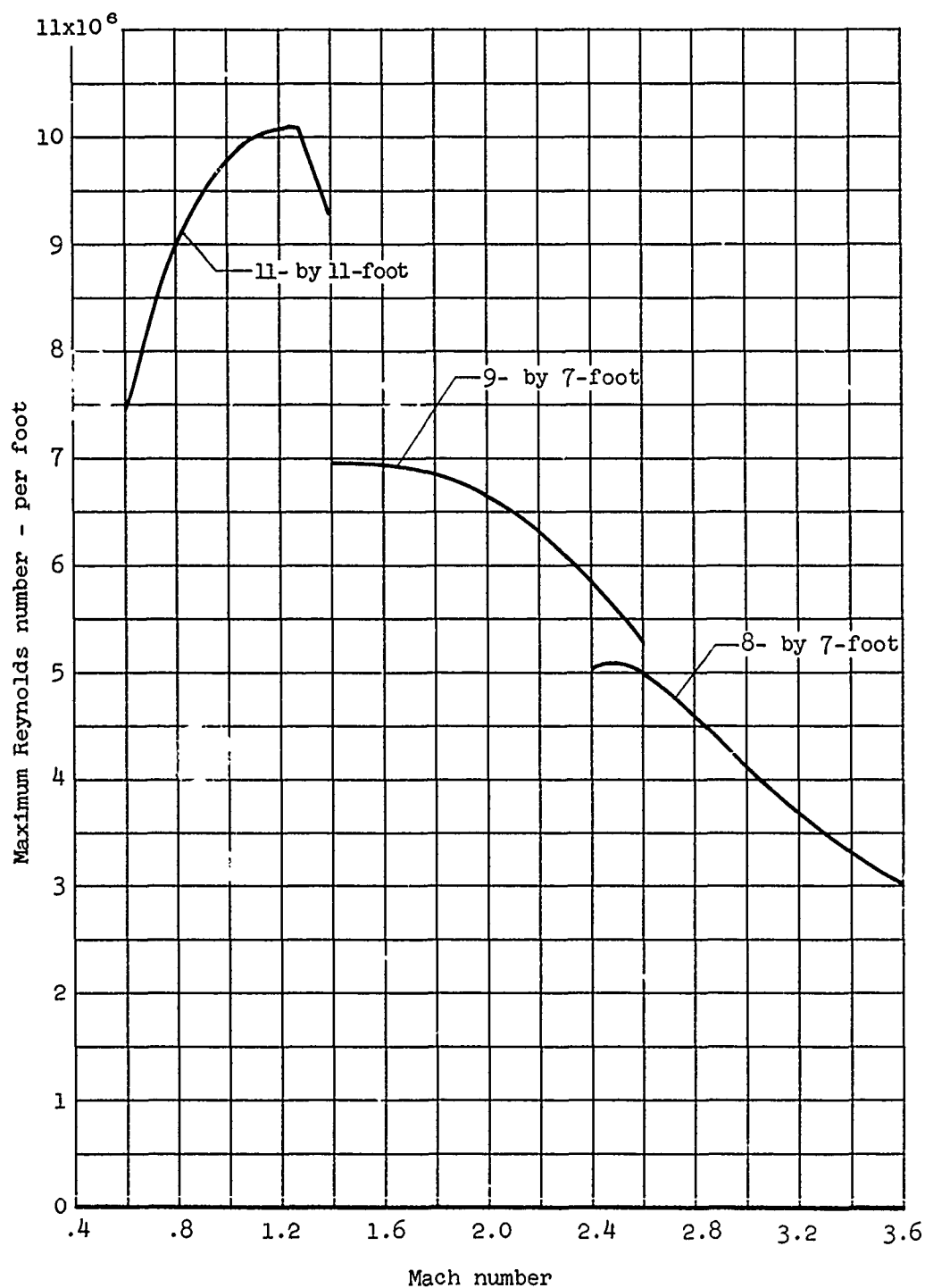
Figure 13. - Maximum operable test section Reynolds number for the three circuits of the Ames Unitary Plan Wind Tunnel.
