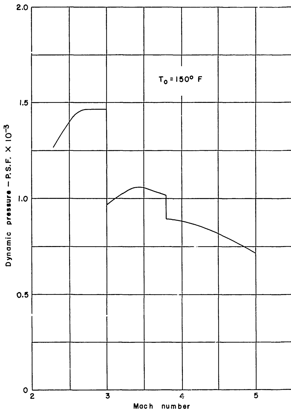
(b) High Mach number test section.
