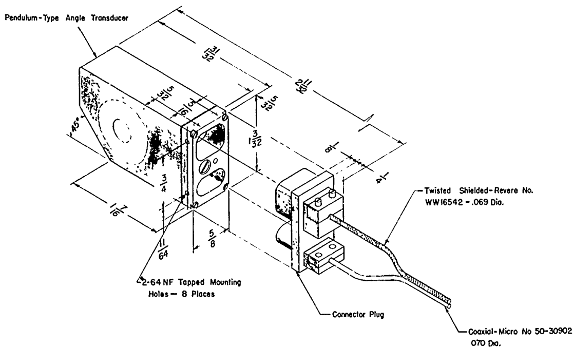
(a) Pendulum-type angle transducer and connector plug.
