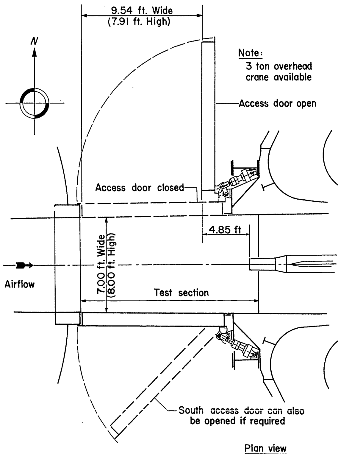
Figure 7. - Access hatch dimensions; 8- by 7-foot supersonic test section, Ames Unitary Plan Wind Tunnel.
