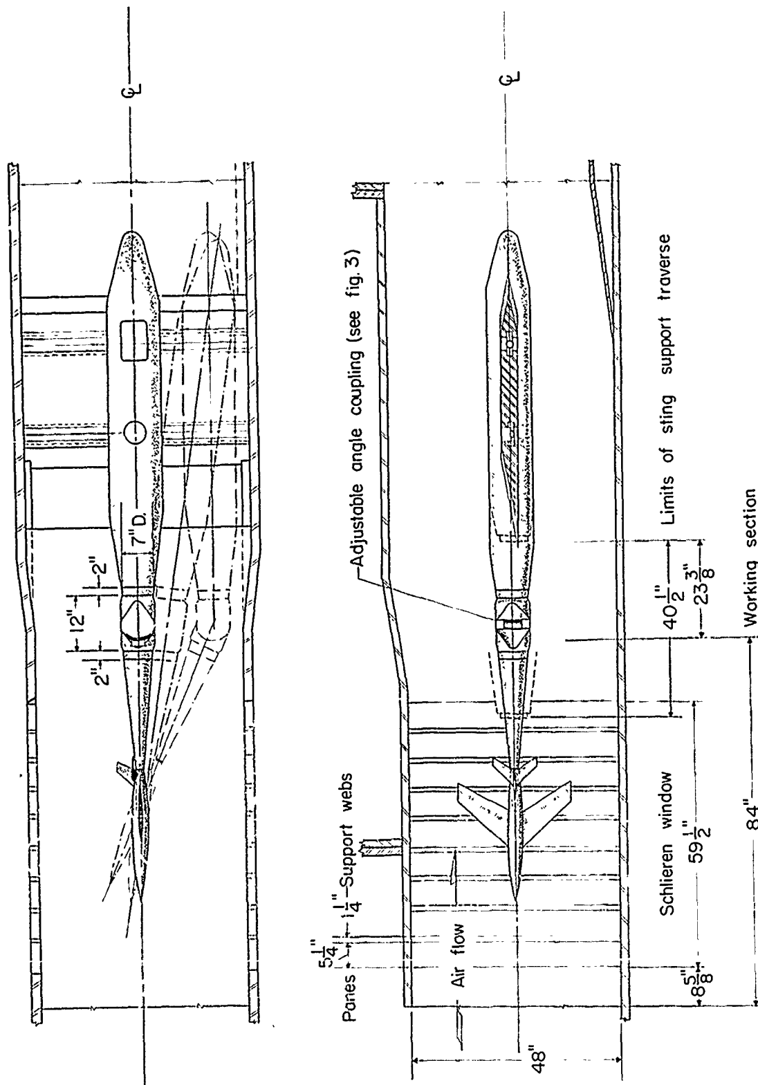
Figure 2.- Test section and basic sting support system, Langley Unitary Plan Wind Tunnel.
