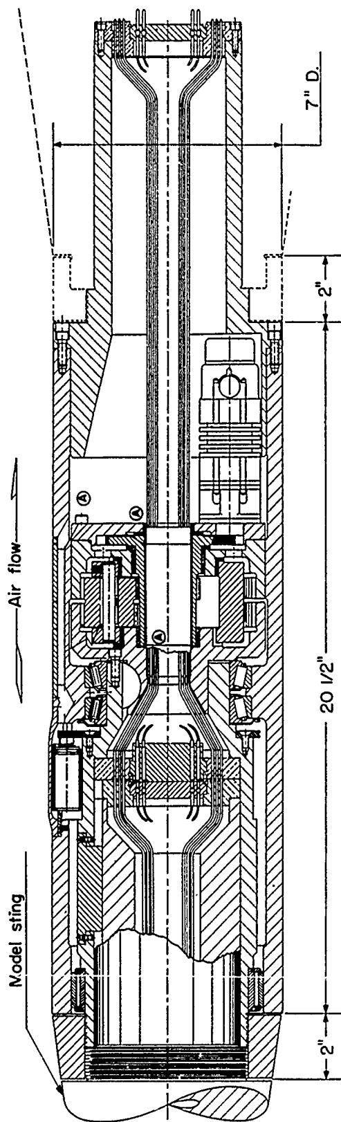
Figure 4.- Rotary coupling, Langley Unitary Plan Wind Tunnel.
