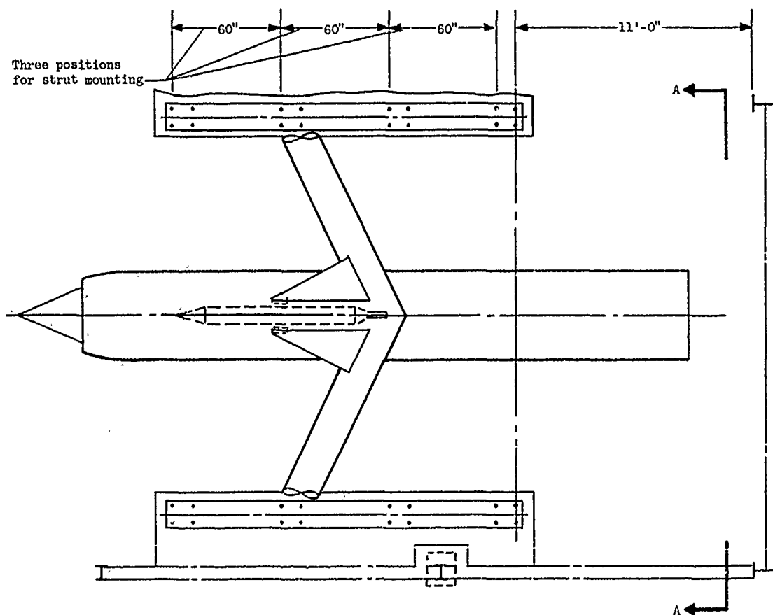
Figure 19.- Shop stand for suspended models, Lewis Unitary Plan Wind Tunnel.
