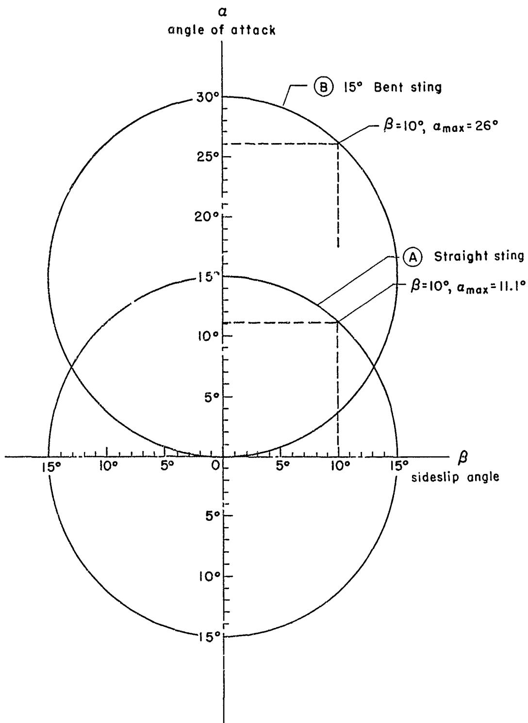
Figure 9. - Angle-of-attack and angle-of-sides ranges, Ames Unitary Plan Wind Tunnel.
