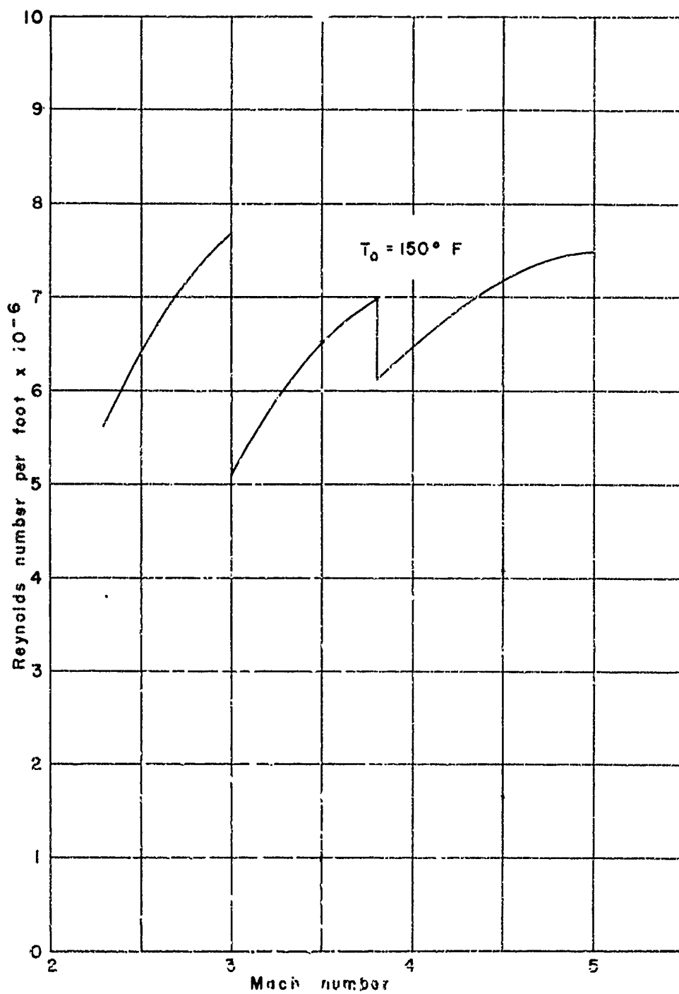
(b) High Mach number test section.
