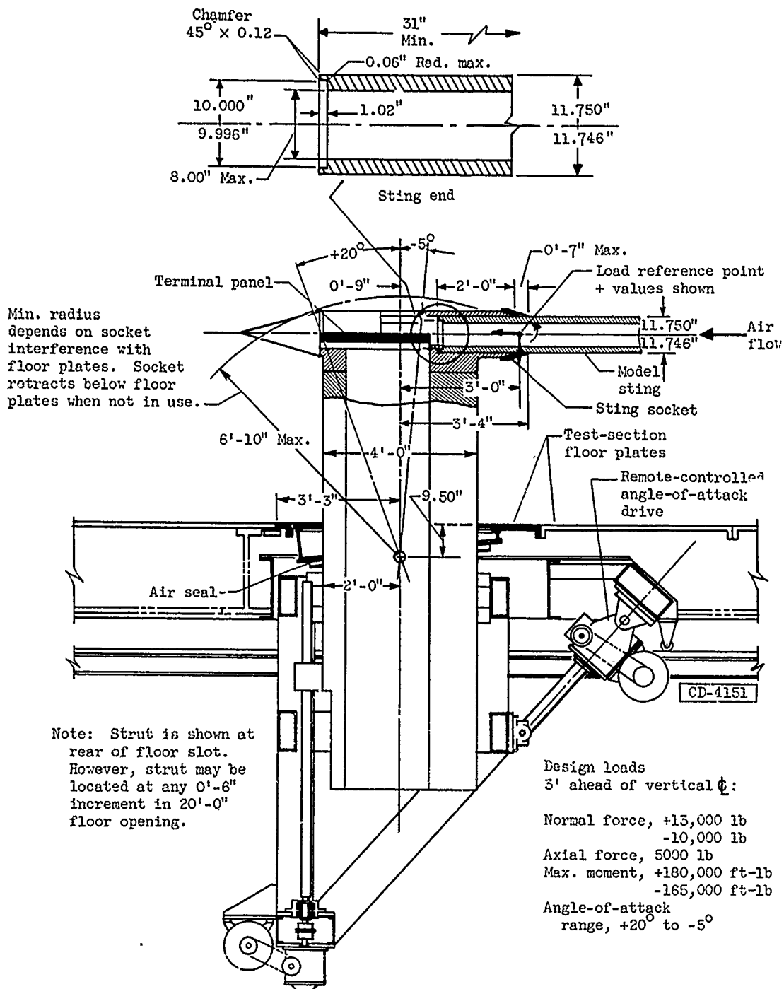
Figure 4. - Sting-mounted model strut, Lewis Unitary Plan Wind Tunnel.
