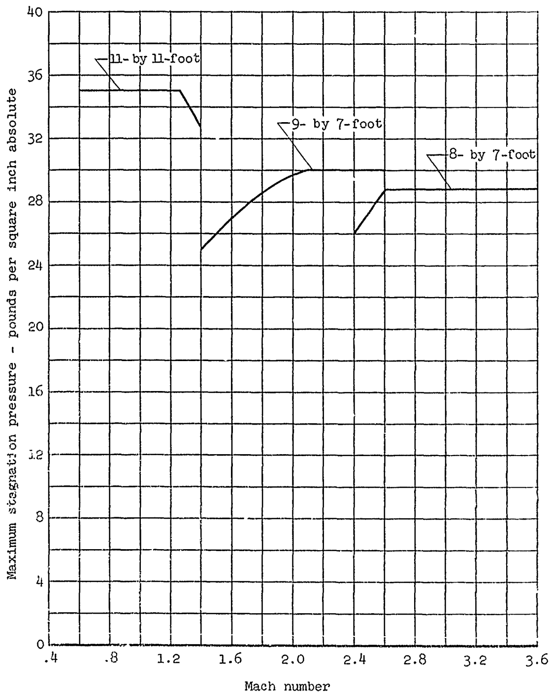
Figure 11. - Maximum operable stagnation pressure for the three circuits of the Ames Unitary Plan Wind Tunnel.
