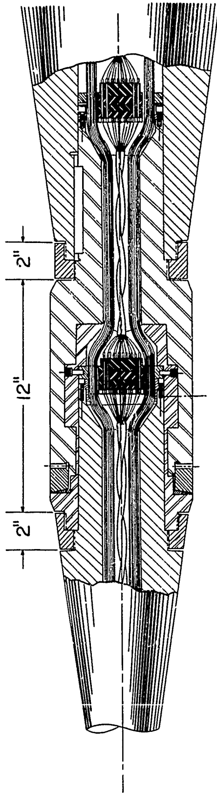
Figure 3. - Adjustable angle coupling, Langley Unitary Plan Wind Tunnel.
