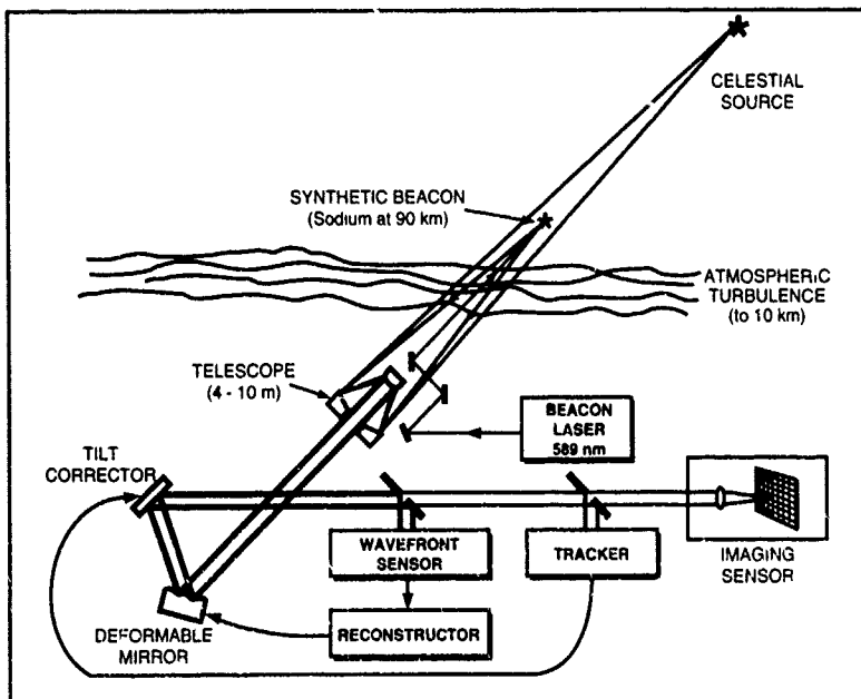
Astronomical applications of adaptive optics with synthetic beacons.
