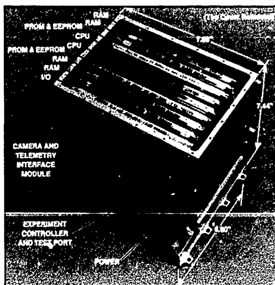
(Right) SBV Signal Processor.
