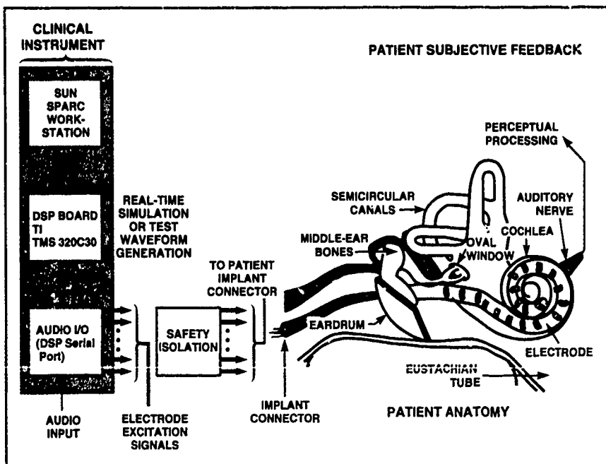
Diagram for the cochlear implant processor.
