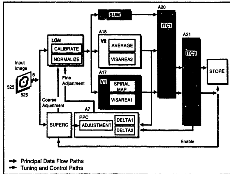
Block diagram of the neural network architecture.
