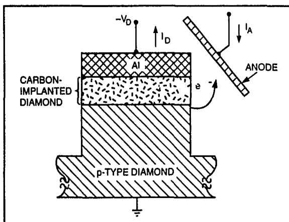
Schematic drawing of the mesa-etched cold cathode diode.
