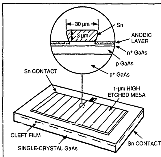
Thin homojunction solar cell.
