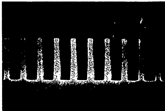
193-nm exposure-0.2 μm resolution.
