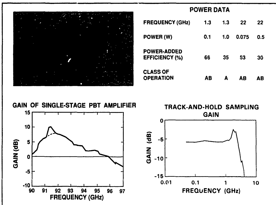
GaAs permeable base transistor.
