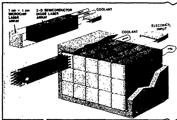
High power, two-dimensional microchip laser array.
