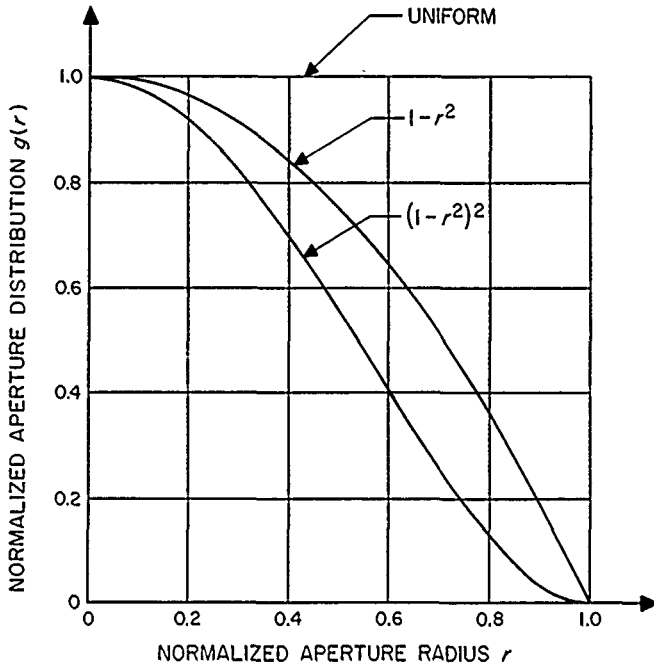
Figure 49. Aperture distributions
