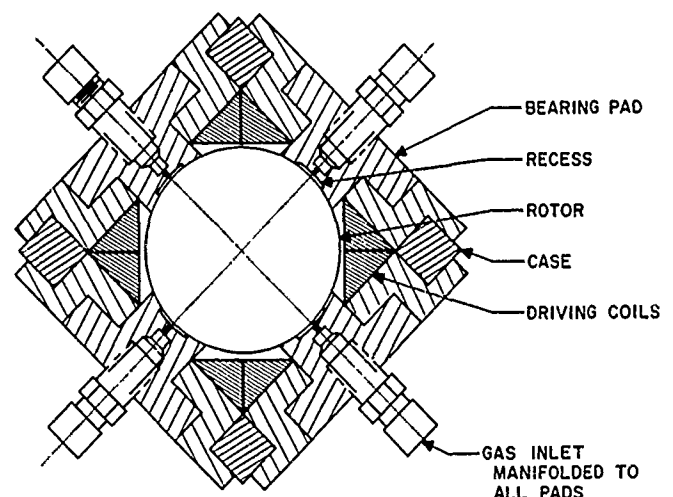
Figure 10. Section drawing of six-pad spinning sphere
