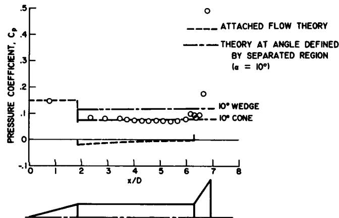
Fig 13 Pressure distribution, 56^\circ flare. Re/\tau_0 = 5.4 \times 10^5
