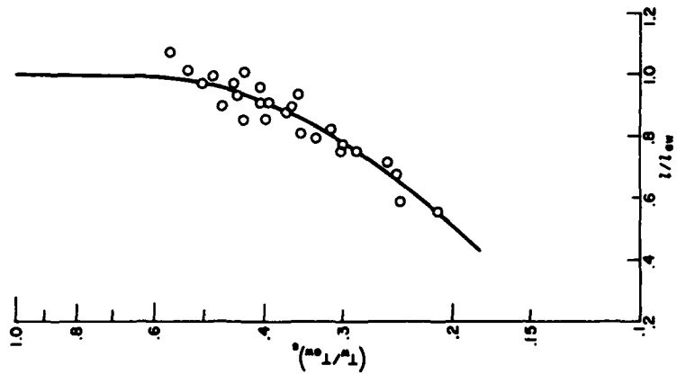
Fig. 7 Effect of wall cooling on the length of separation. \theta = 24^\circ ; 1.0 \times 10^5 \leq Re/Re_0 \leq 5.0 \times 10^7
