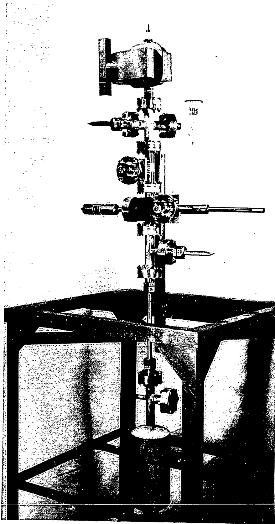
Fig. 41. Stainless-steel vacuum system.
