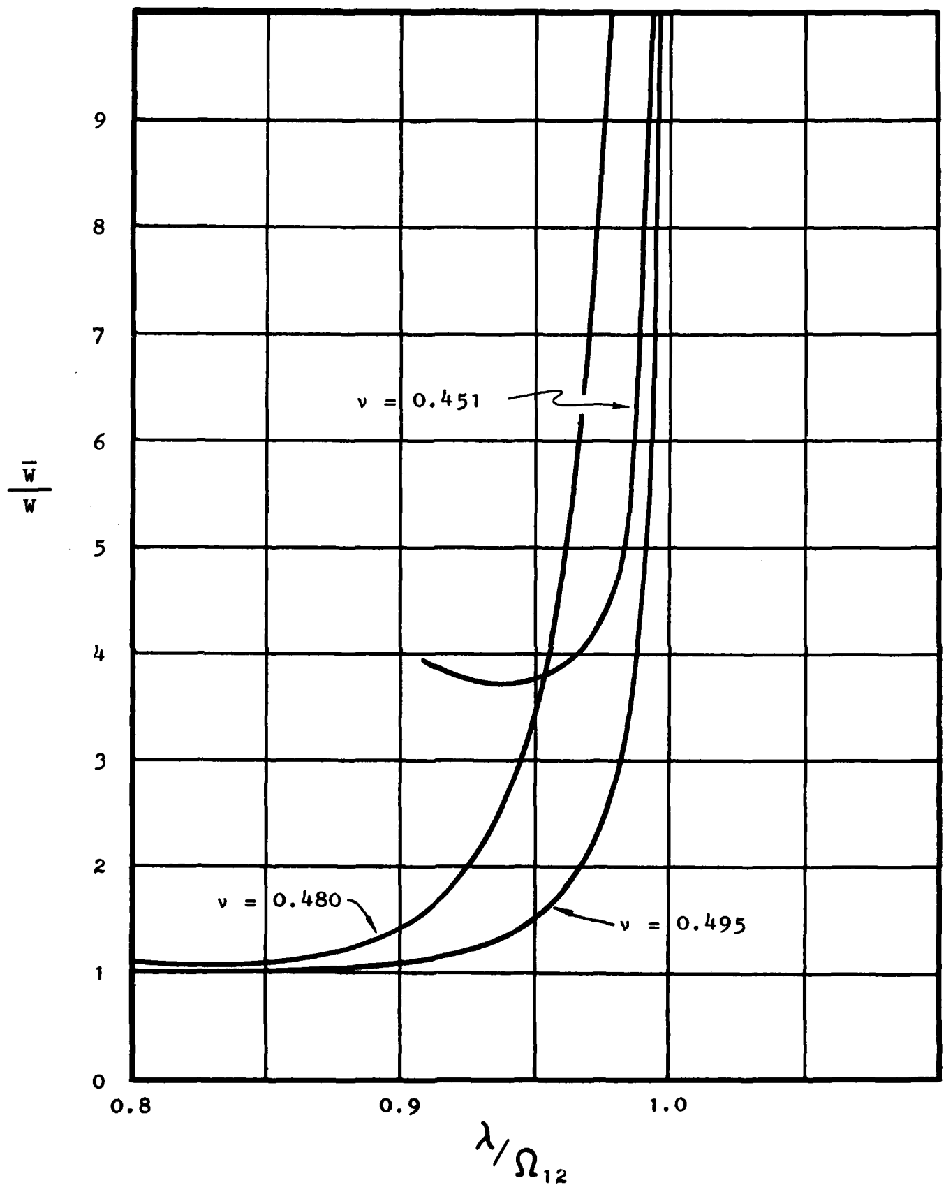
Figure 2(b) Amplitude ratio-frequency plots in the neighborhood of the second resonance for forced transverse vibrations of a solid, elastic core case-bonded to an infinitely-long, rigid cylinder
