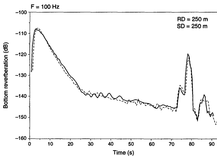
Figure 19 Monostatic reverberation from the bottom - solid line (average of five frequencies) compared to the reverberation from MOCASSIN (dashed line).
