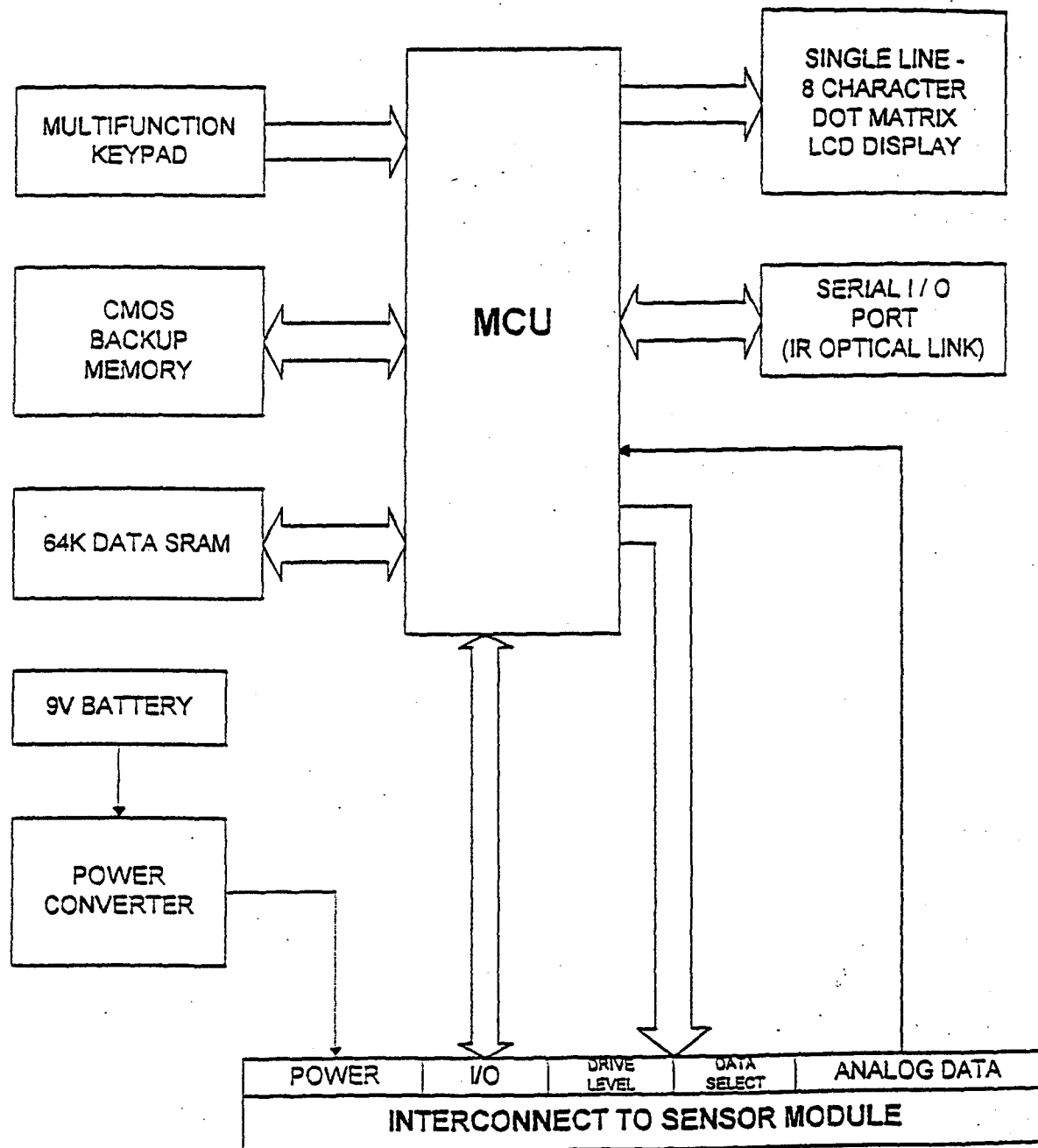
Figure 14. Block Diagram of System Support Module
