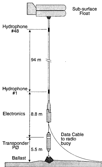
Figure 2 The SACLANTCEN vertical array as deployed in a bottom-moored configuration.
