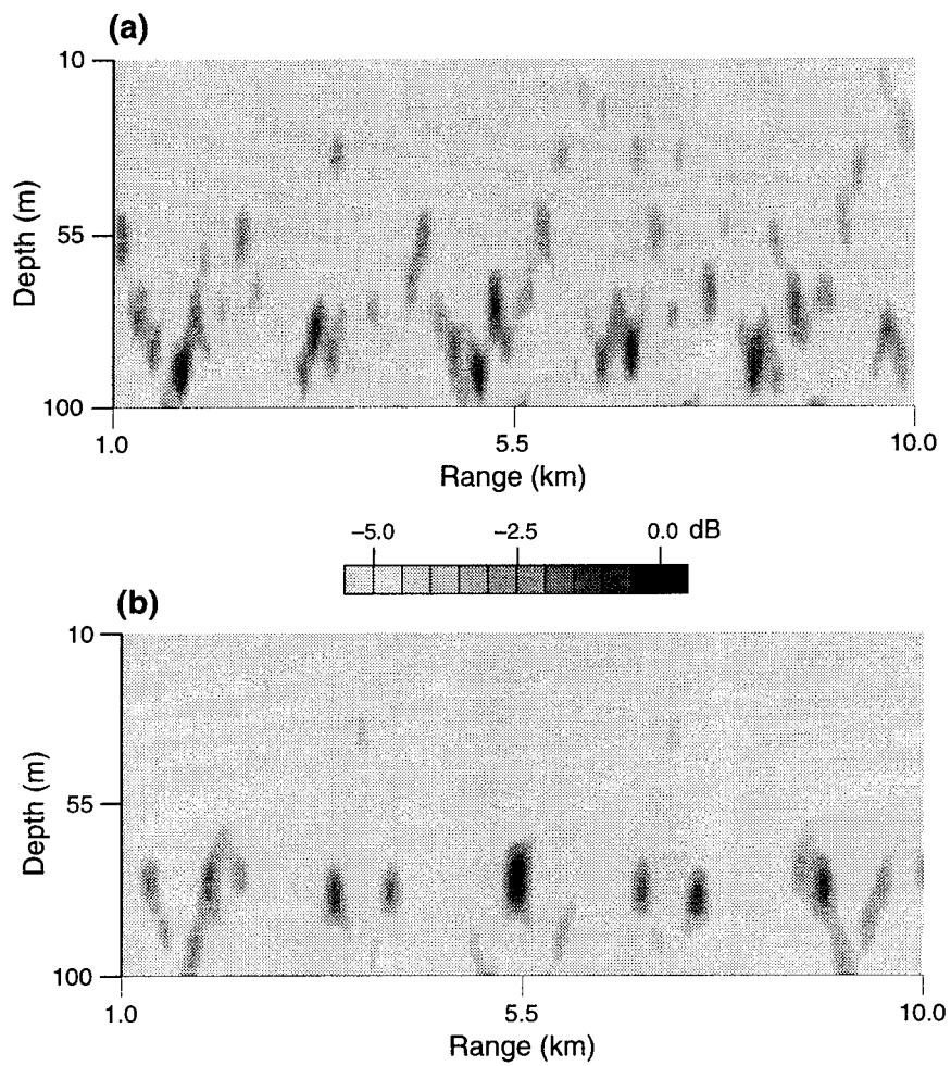
Figure 8 Range/depth ambiguity surface for the stationary source using (a) baseline model and (b) GA estimated model, at T = 0 min.
