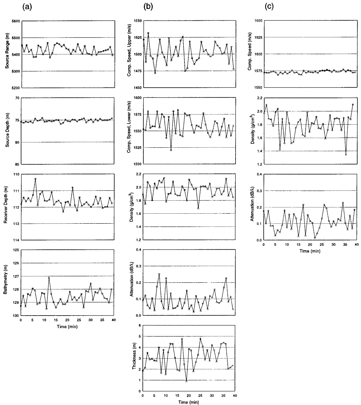
Figure 5 Mean of the GA parameter estimates as a function of time: (a) geometric, (b) sediment, and (c) bottom parameters.
