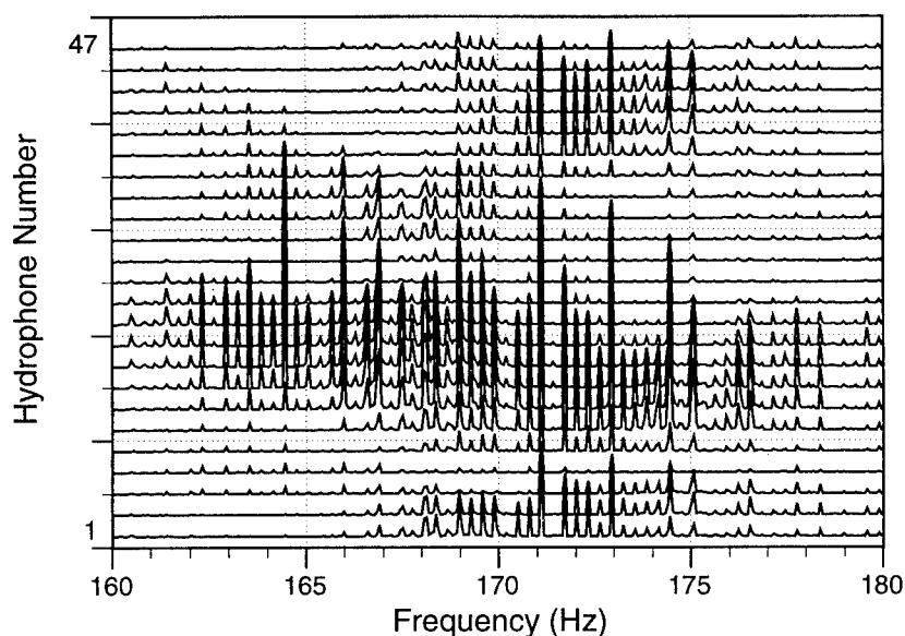
Figure 3 Spectrum for the stationary source PRN signal as received on the vertical array at T = 0 min, odd-numbered hydrophones only.
