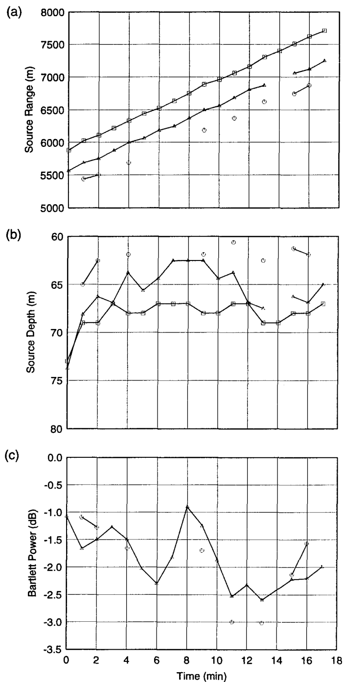
Figure 9 Source locations and Bartlett power as a function of time. Actual source locations (squares), estimated source locations based on GA estimated model (triangles) and estimated source locations based on baseline model (circles) for the moving source: (a) range (b) depth and (c) Bartlett power.
