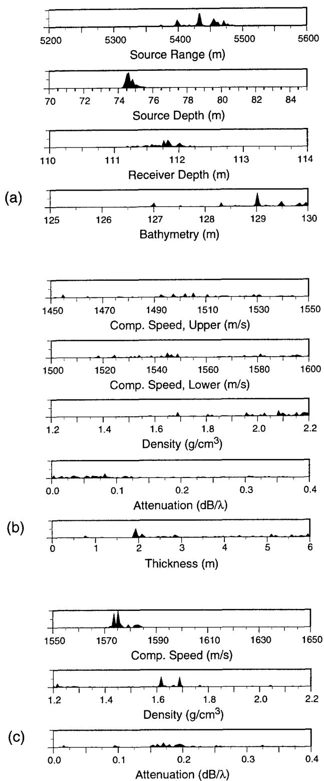
Figure 6 A posteriori probability distributions for each of the 12 model parameters based on the 40 observations: (a) geometric, (b) sediment, and (c) bottom parameters.
