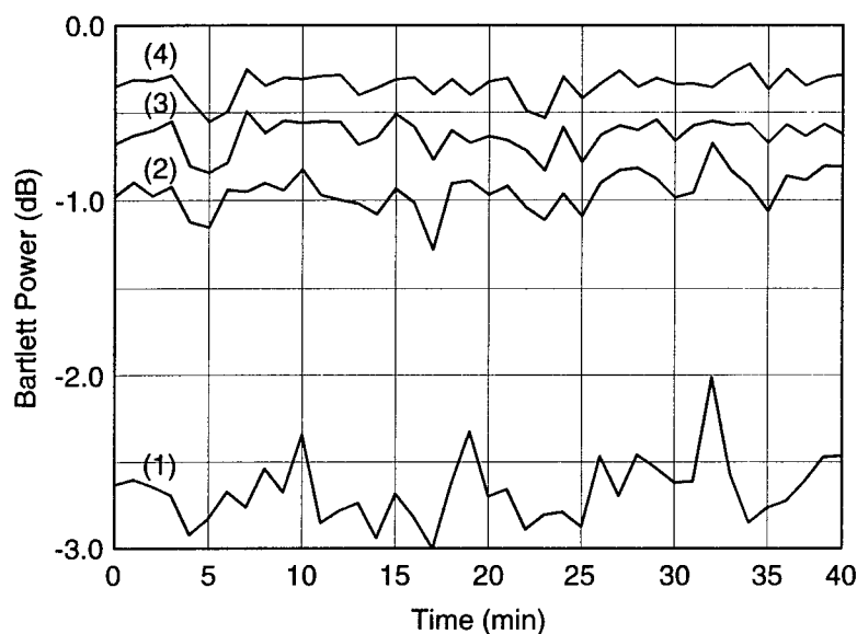
Figure 7 Bartlett power at the surface maximum as a function of time for the stationary source using (1) baseline model, (2) baseline with GA estimated bathymetry 128.9 m and receiver depth 111.7 m, (3) baseline with GA estimated bathymetry 128.9 m, receiver depth 111.7 m and sediment parameters, (4) all GA estimated parameters (search region 5–6 km, 10–100 m).
