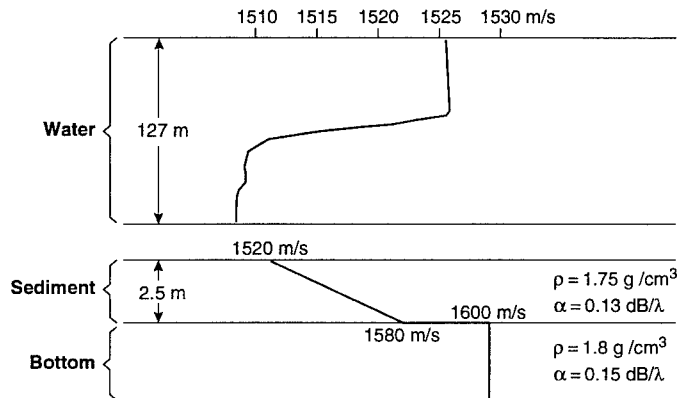
Figure 4 Measured sound-speed profile and bathymetry with historical geoacoustic parameters for the North Elba experiment site, geoacoustic parameters are from Ref. [16].
