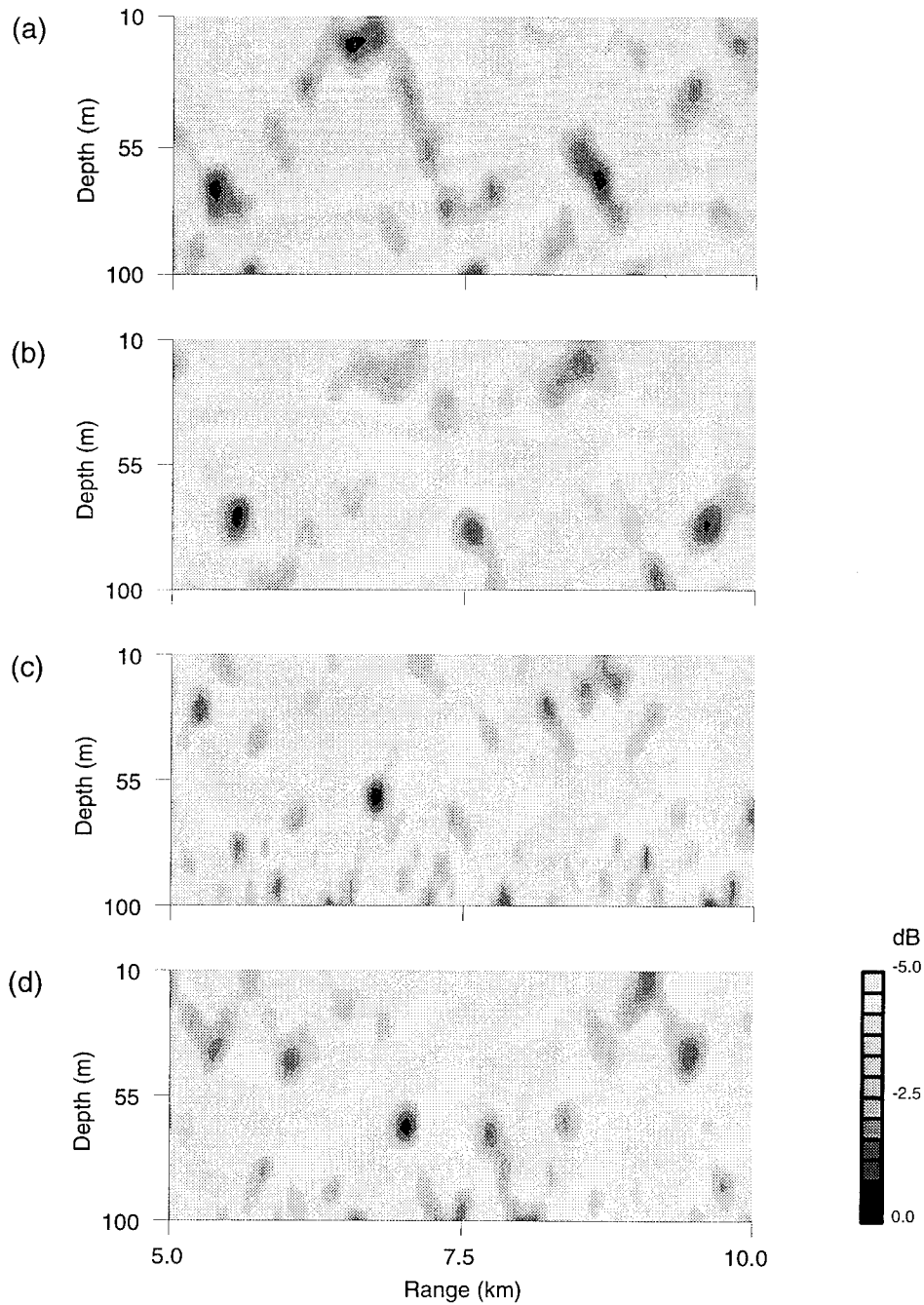
Figure 10 Range/depth ambiguity surfaces for the moving source calculated using the baseline and GA estimated models of Table 2: (a) baseline model at T = 0 min, (b) GA estimated model at T = 0 min, (c) baseline model at T = 15 min, (d) GA estimated model at T = 15 min.
