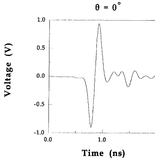
Figure 2.3: Measured sensor waveform for 200 mm diameter ground plane.
