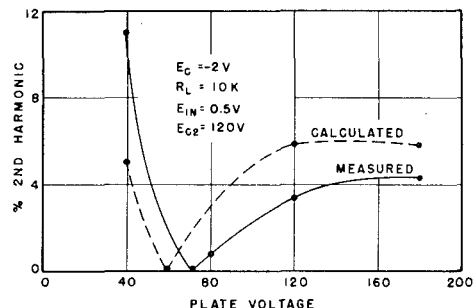
Figure 3 - Comparison of measured and calculated values of second-harmonic distortion in 6AK5 as amplifier
