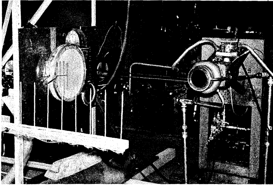
Figure 1 - Thermocouple setup at motor test stand
