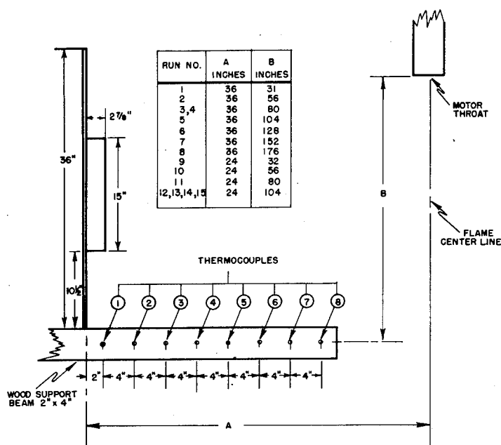
Figure 3 - Plan position of thermocouples
