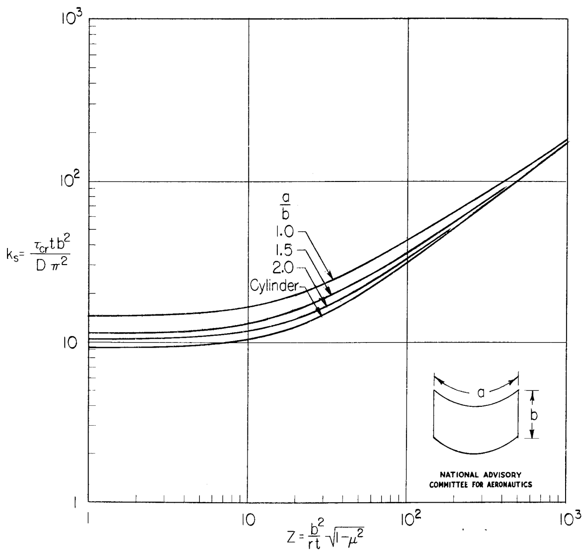
Figure 6.- Estimated theoretical critical-shear-stress coefficients for curved panels with clamped edges and having circumferential length greater than axial length.
