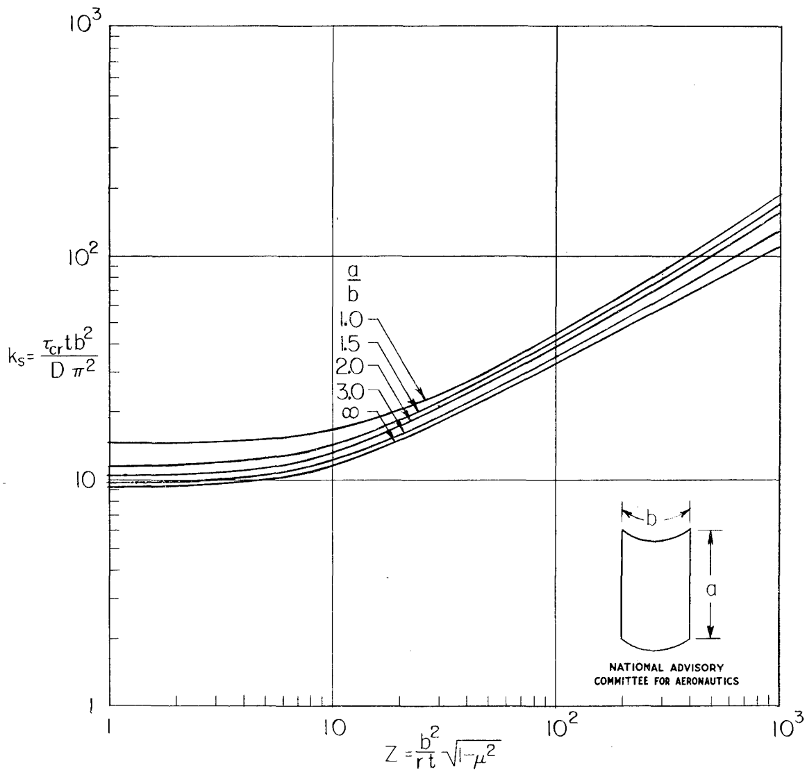
Figure 7.- Estimated theoretical critical-shear-stress coefficients for curved panels with clamped edges and having axial length greater than circumferential length.
