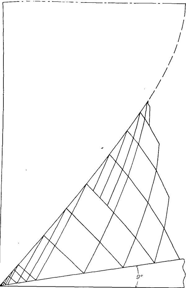
FIGURE 9.—Practical system of calculating the internal-supersonic-flow properties for a slender open-nose body of revolution for M=1.6 .
