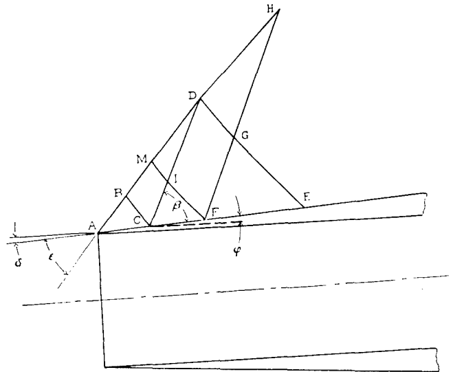
FIGURE 3.—Practical system of calculating the flow field for a slender open-nose body of revolution.
