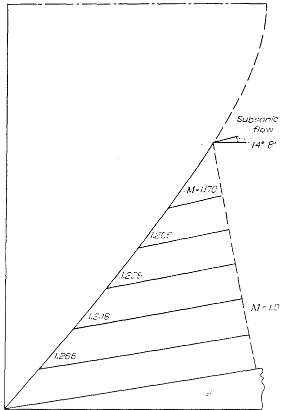
FIGURE 10.—Calculated streamlines and shock wave for internal flow in a slender open-nose body of revolution for M=1.6 .
