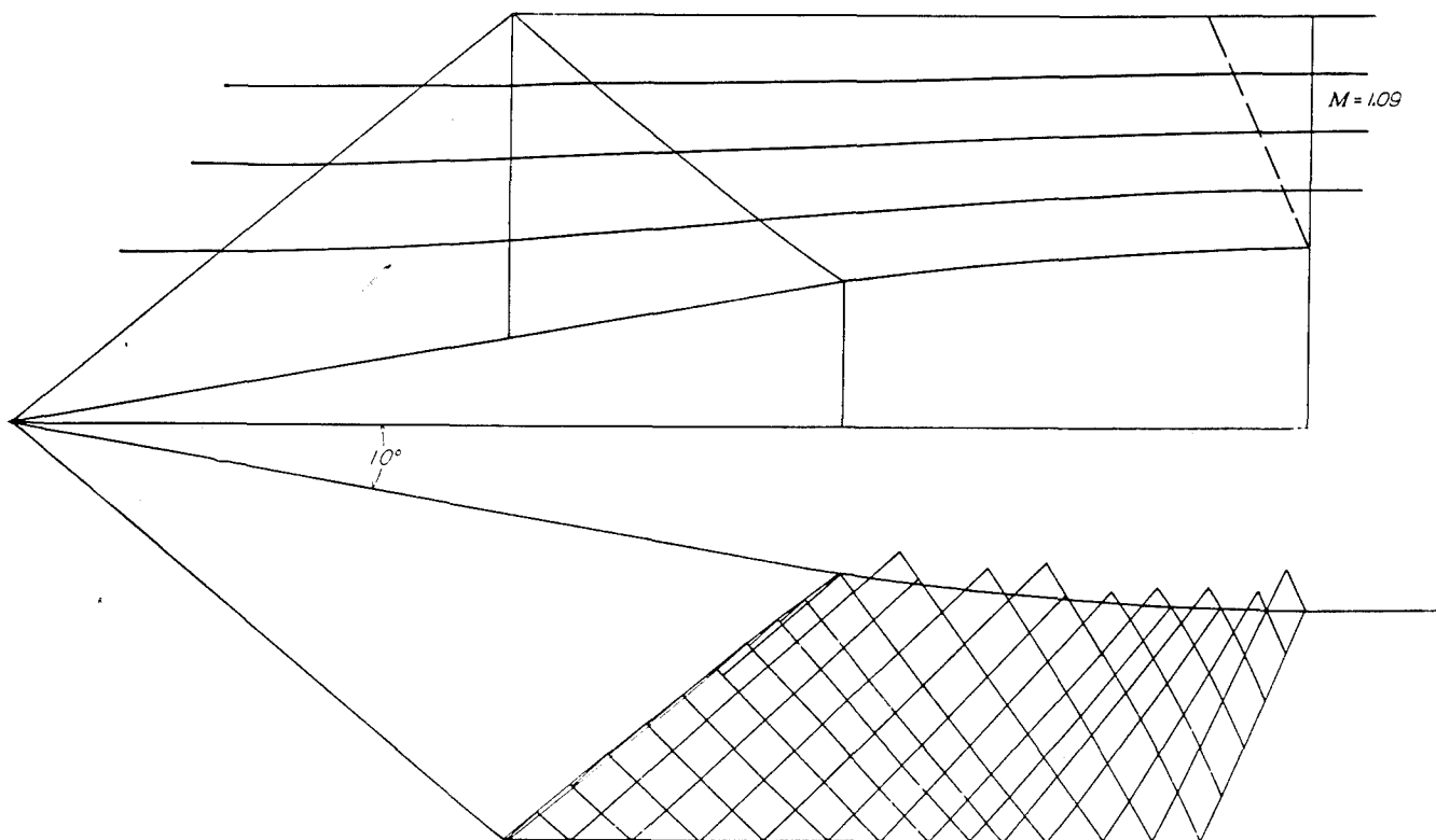
FIGURE 14.—Practical system of calculating the shape of the central body, of the streamlines, and of shock-wave shape for a supersonic inlet at M=1.09 .
