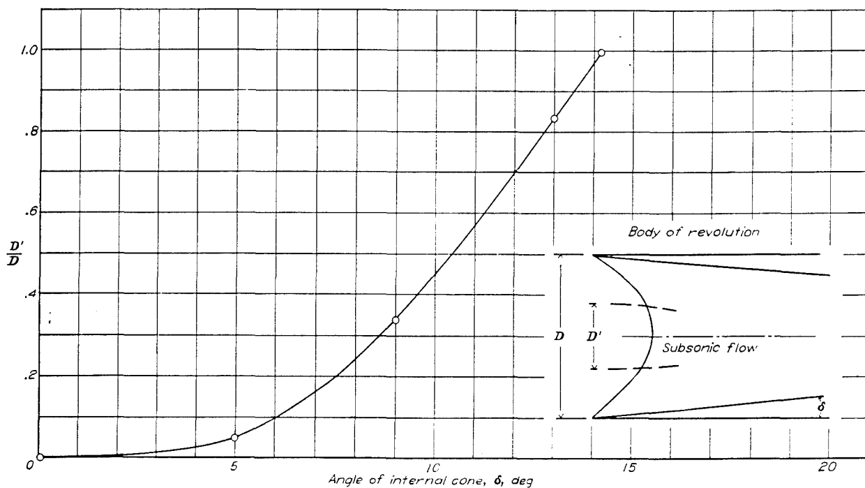
FIGURE 13.—Ratio of the diameter of the region in which strong shock occurs to the diameter of the inlet as a function of the angle of internal cone. M=1.6 .
