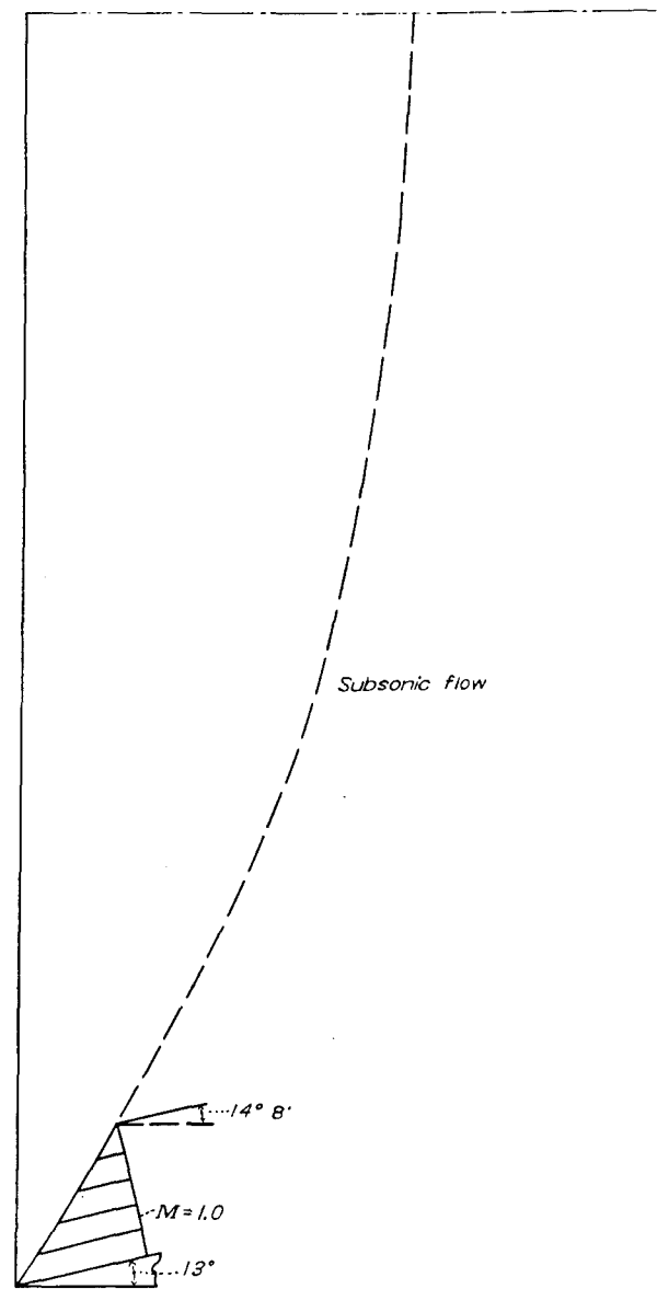
FIGURE 12.—Calculated streamlines and shock wave for internal flow in a slender open-nose body of revolution for M=1.6 .
