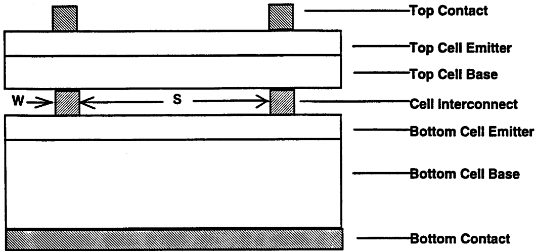
Figure 5.1. Schematic cross-section of mechanically stacked tandem solar cell. S is the spacing of the interconnect grid, and W is the grid line width. The top cell is a very thin ( 5\ \mu\text{m} ) AlGaAs or GaInAsP junction. The bottom cell is made of Si.
