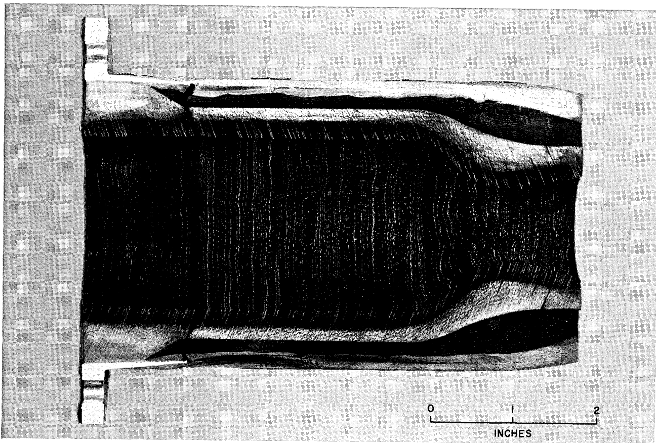
Fig. 22. Cross section of HITCO ablative chamber, showing the area of separation
