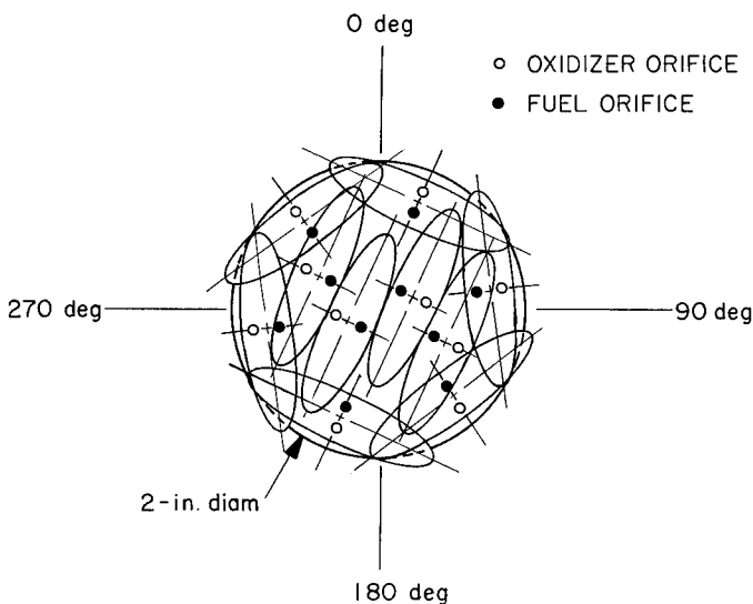
Fig. 1. Arrangement of the 10 pairs of propellant orifices and resulting sprays from the Mod IV 100-lb-thrust injector
