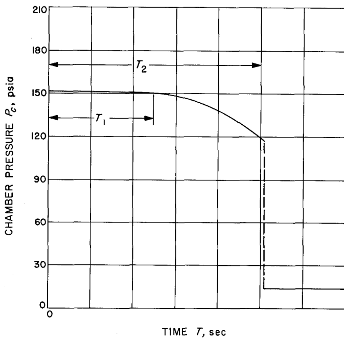
Fig. 11. Characteristic plot of pressure in an ablative chamber as a function of test duration
