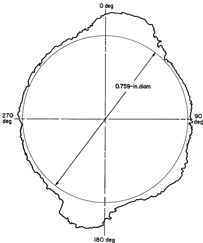
Fig. 17. Nozzle-throat area in AVCO ablative chamber, before and after the firing test
