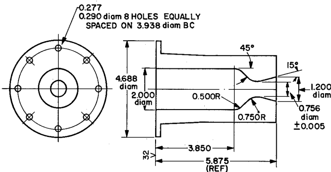
Fig. A-1. Control drawing of 100-lbf-thrust chambers
