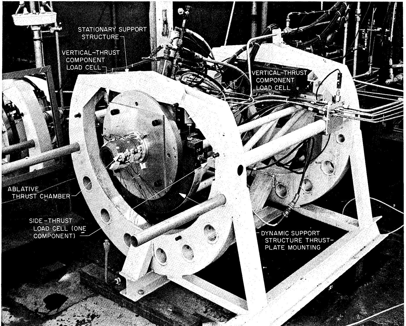
Fig. 3. Six-component thrust-measuring system
