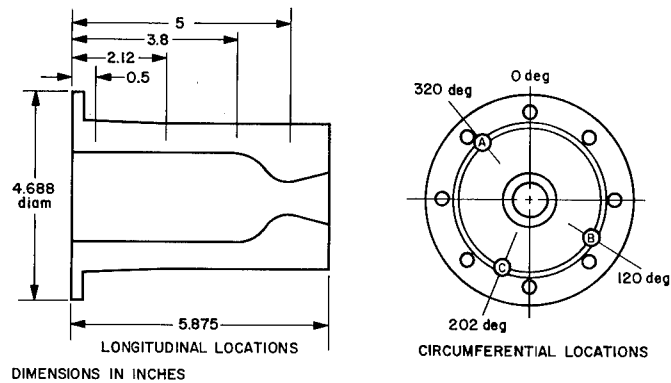
Fig. 4. Thermocouple locations on the ablative chambers
