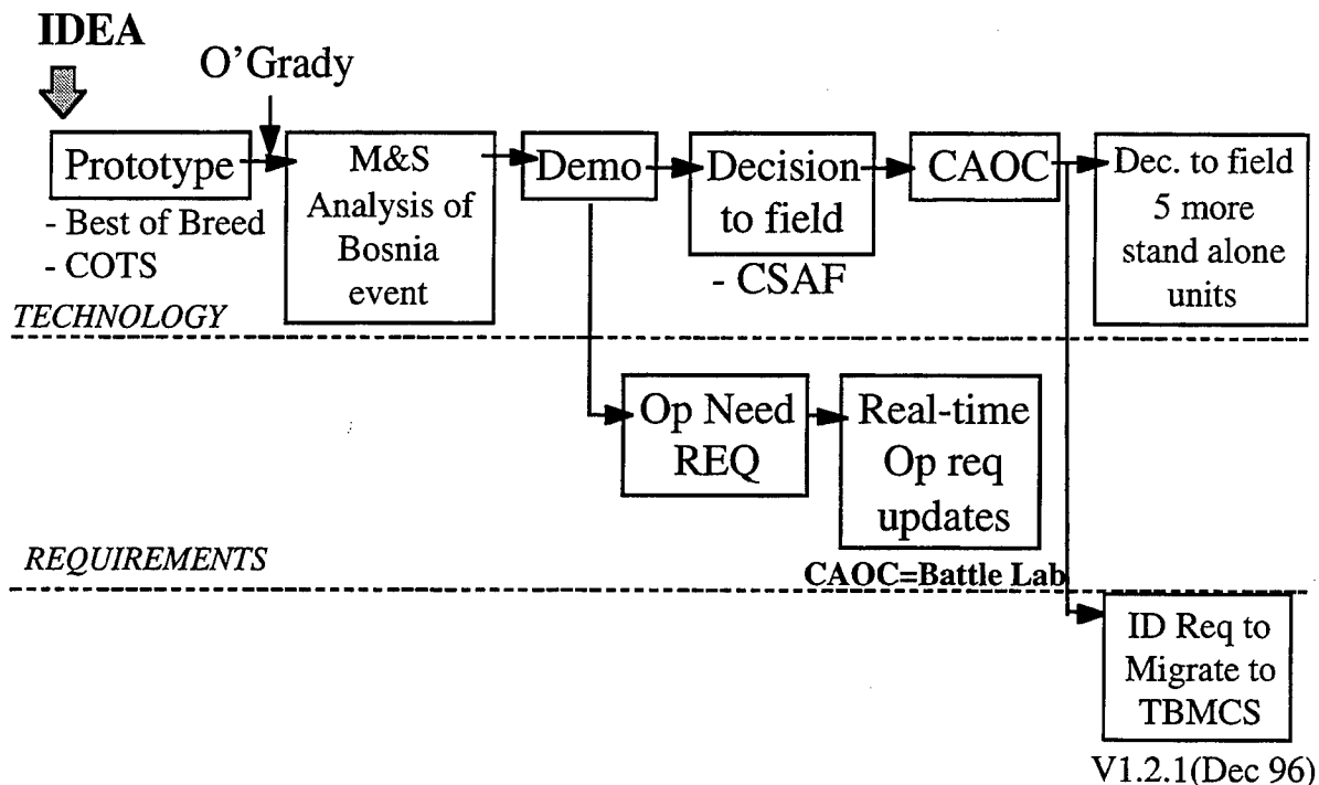
Figure 5-7. JSAS Example—History
