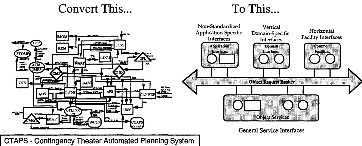
Figure 5-5. CORBA Encapsulation
