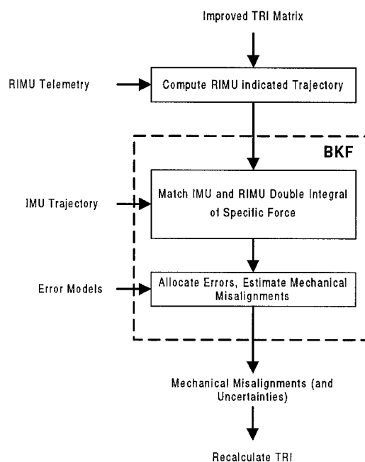
Figure 7. RIMU Boost Alignment Process
