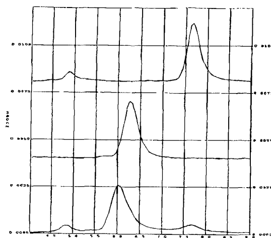
Figure 4. Analytical gel filtration analysis of gp120-sCD4 binding. Samples were injected onto a G3000SW XL column (Toso-Haas) run at 1ml/min in PBS buffer. Top: 5 µg sCD4; middle: 10µg HIV-1 LAI gp120; bottom: 5 µg sCD4 + 10 µg HIV-1 LAI gp120 pre-incubated for 1 hr at 4 °C.
