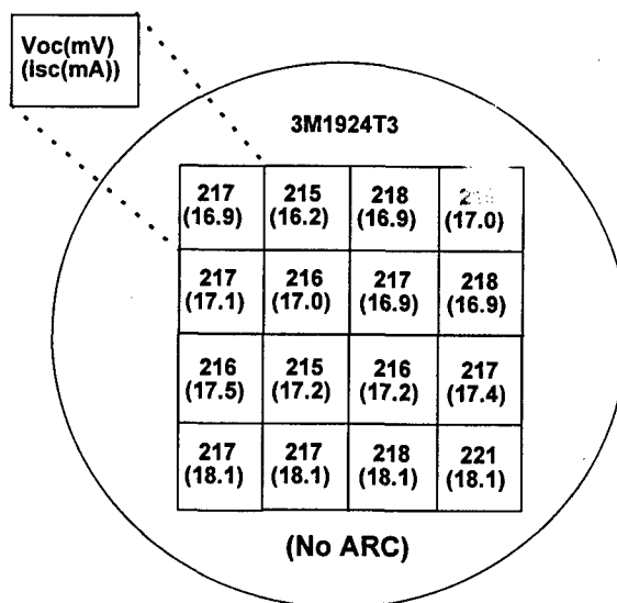
Figure 19. Voc and Isc distribution of 1 cm x 1 cm Ge single junction cells (without ARC) across a 3" diameter substrate.
