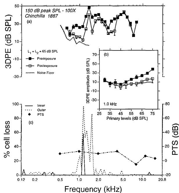
Figure 18. (a) The pre- and 30-day postexposure DPEgrams, (b) the pre- and 30-day postexposure 3DPE I/O function measured at 1.0 kHz, and (c) the cochleogram and PTS audiogram (symbols) for Chinchilla 1887 exposed to the 150 dB peak SPL, 100X, reverberant impulses.
