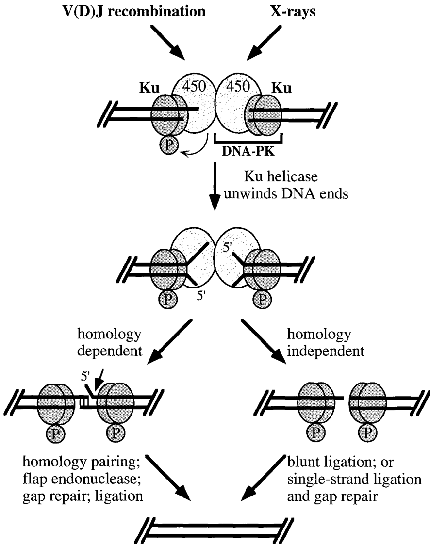
Fig. 5. Model for Ku in DSB repair. Free DNA ends are created by X-rays or as intermediates in V(D)J recombination. DNA-PK \zeta has an alignment function and autophosphorylates Ku to give Ku helicase activity. Ku helicase unwinds the DNA ends, which can then be joined by homology dependent or homology independent mechanisms (see Fig. 3). The overall joining reaction is non-conservative and may involve the loss of nucleotides
