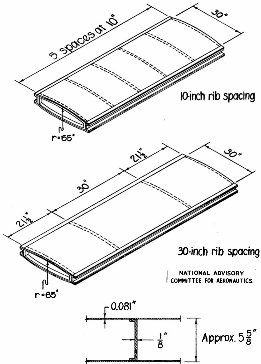
Section of rib at center line of panel
