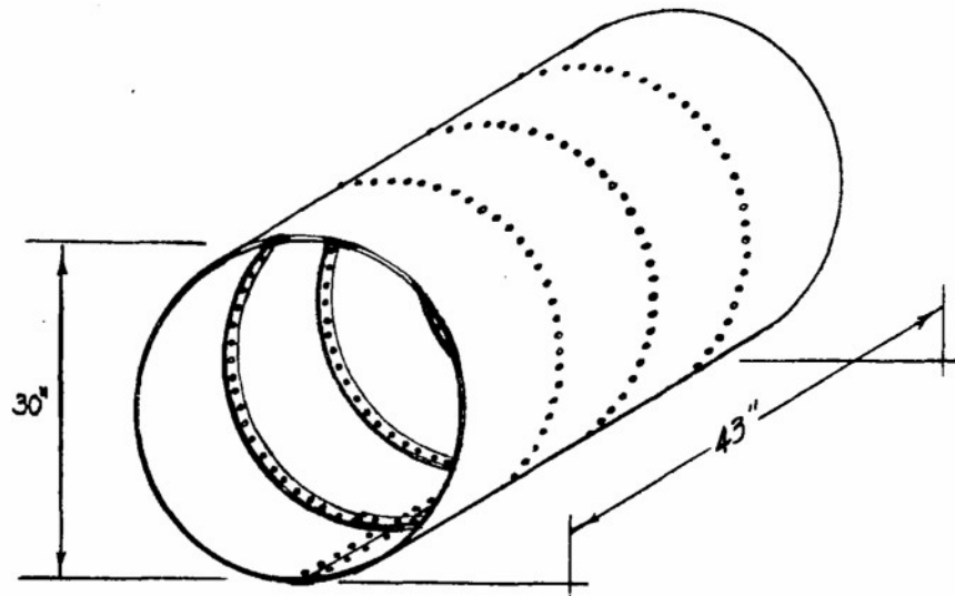
Figure 1. - Test specimens.
