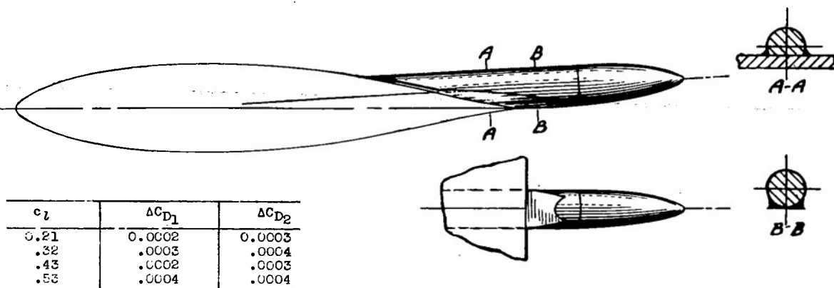
Figure 18. - Fillet M; \beta , 3.25^\circ a , 0.2088c; b , 0.0729c; R , 6 \times 10^6 (approx.)
