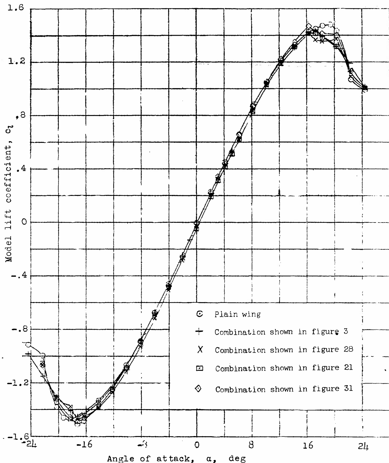
Figure 34.- Typical lift characteristics of NACA 65,3-018 airfoil section with pusher-propeller shaft combinations; R, 6 \times 10^6 (approximately).
