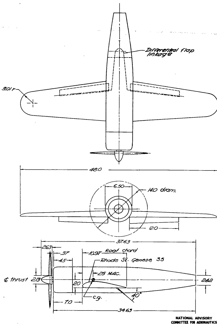
Figure 6.- Three-view sketch of powered test model as tested in Langley free-flight tunnel. Wing incidence \cdot 0^\circ ; dihedral angle \cdot 0^\circ ; all dimensions in inches.
