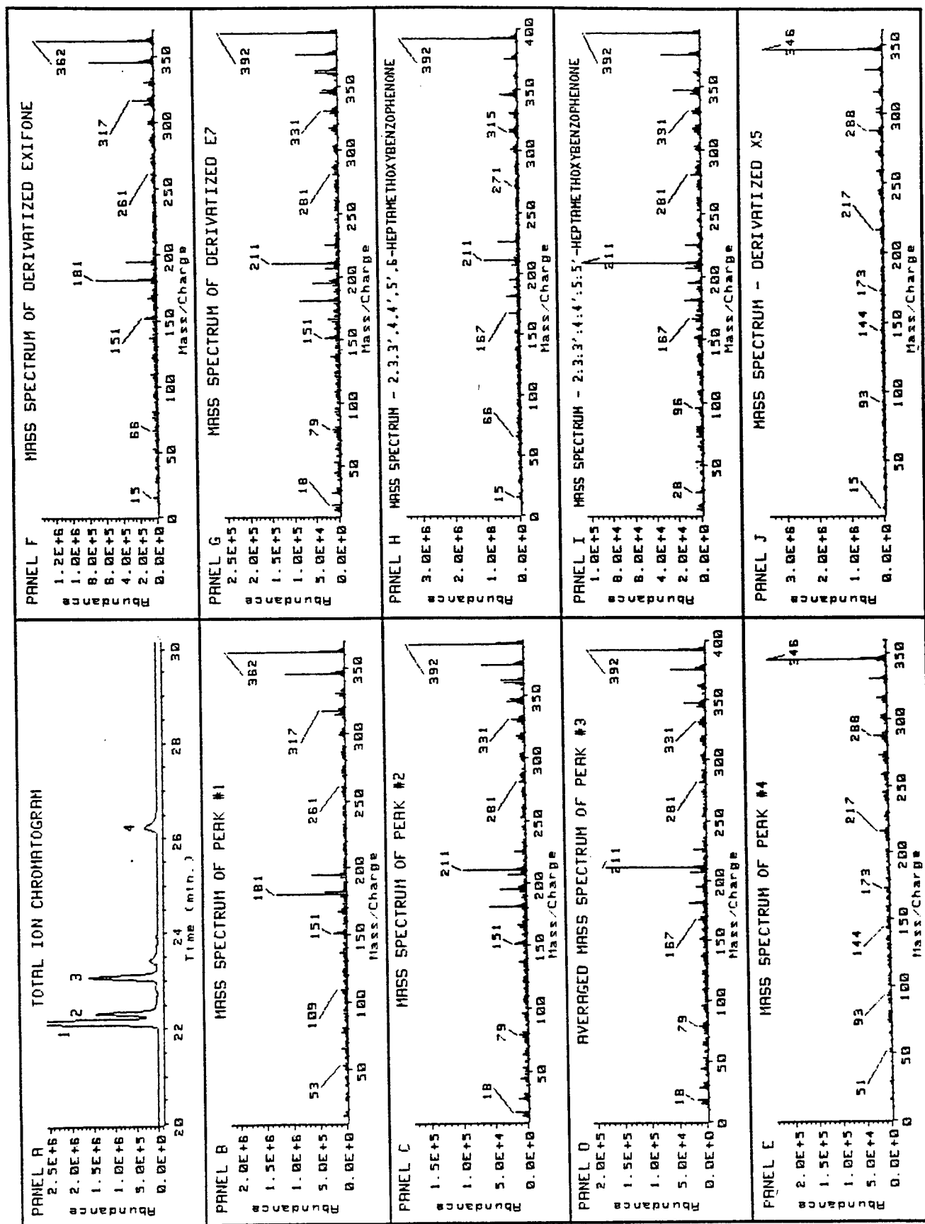
Figure 8. Panels A-J. Conversion of exifone into pentahydroxyanthrone (X5) under conditions of the Fenton reaction as detected by GC-MS (derivatized to their corresponding permethyl ether form prior to injection). Panels: A. total ion chromatogram of reaction products, B. mass spectrum of peak #1, C. mass spectrum of peak #2, D. mass spectrum of peak #3, E. mass spectrum of peak #4; Standards: F. mass spectrum of derivatized exifone, G. mass spectrum of derivatized E7, H. mass spectrum of 2,3,3',4,4',5',5'-heptamethoxybenzophenone, I. mass spectrum of 2,3,3',4,4',5',5'-heptamethoxybenzophenone, and J. mass spectrum of derivatized X5.
