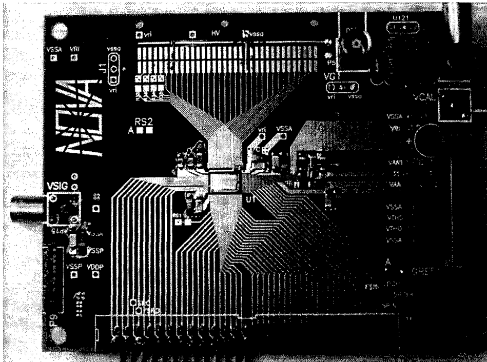
Photograph 5 A photograph of new printed circuit board for RENA chip mounting
