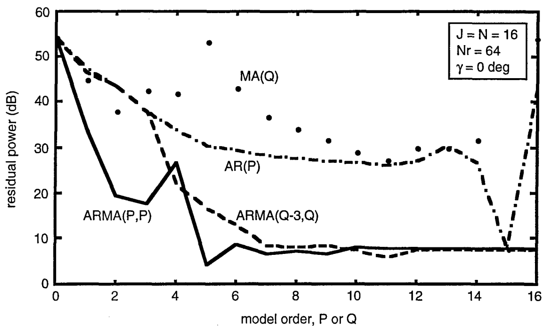
Figure 4-2. Residual power as a function of model order for 2-D MA, AR, and ARMA models ( J = N = 16 ; N_{rd} = 64 ; \gamma = 0 \text{ deg} ).
