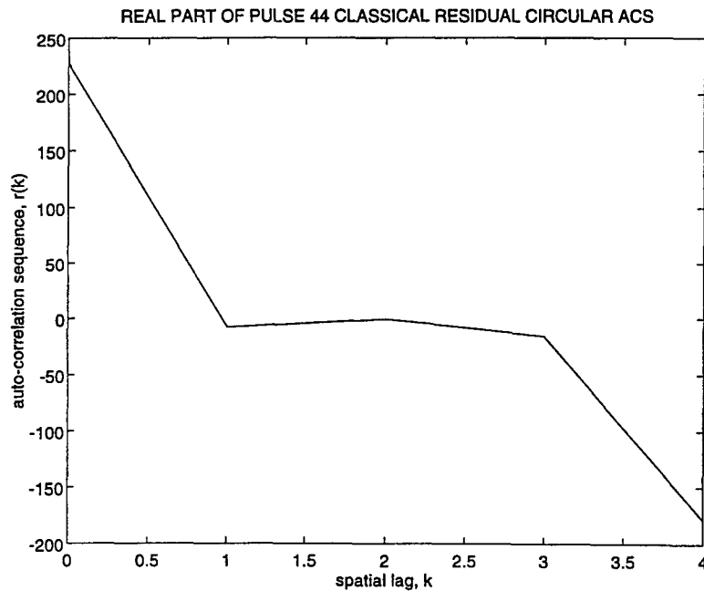
Figure 4-19. Real part of pulse 44 joint-domain residual circular ACS versus spatial lag ( \gamma=20 deg).
