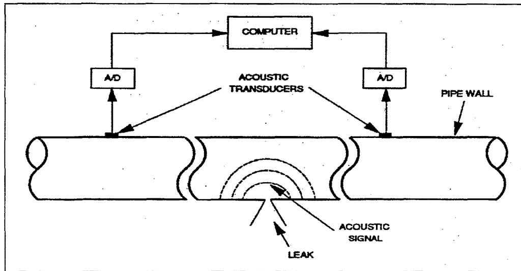
Figure 9. Acoustic emission leak detector.
