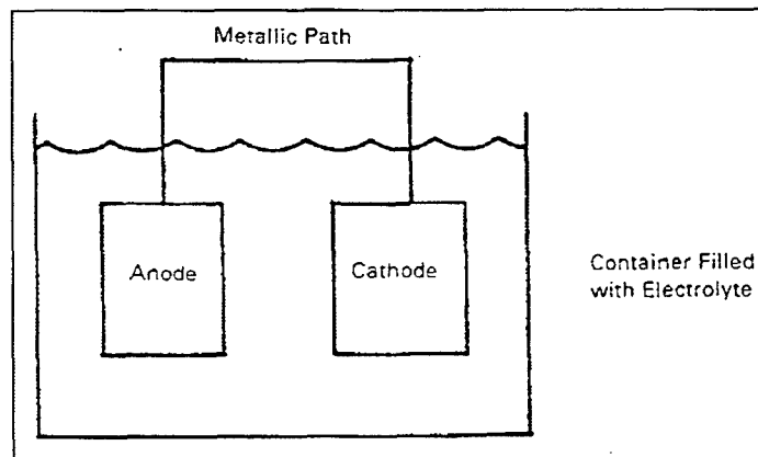
Figure 10. The electrochemical cell.
