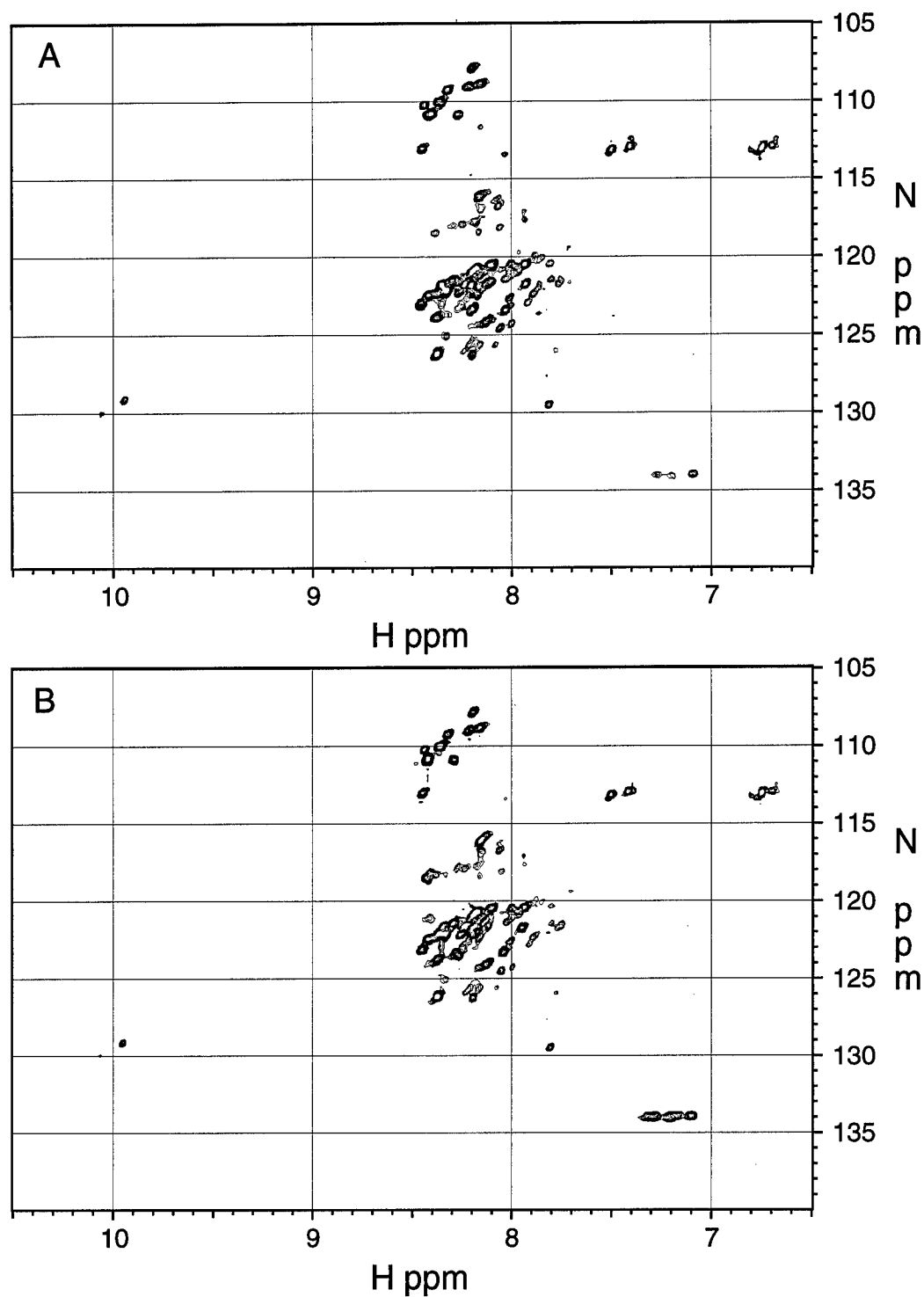
Figure 3. ^1\text{H} , ^{15}\text{N} HSQC spectra of free ^{15}\text{N} -hER[253-341] (A) and ^{15}\text{N} -hER[253-341] in the presence of the phosphopeptide. The protein and peptide concentrations were approximately 0.1 and 0.3 mM, respectively.
